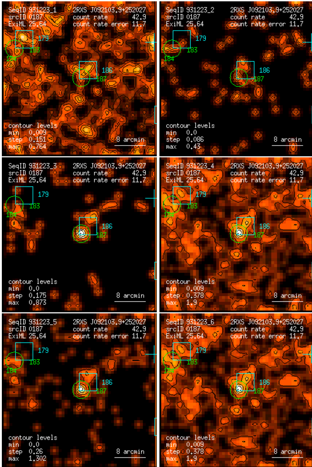
Figure 187: RASS 931223: detection 0187: band rate images, Gaussian filter: (1) PSPC channels 11 – 41, (2) 52 – 90, (3) 91 – 201, (4) 11 – 235, (5) 52 – 201, (6) 11 – 201. Broad band rates in counts/ks. Band rate contour levels in counts/ks/arcmin 2 .
