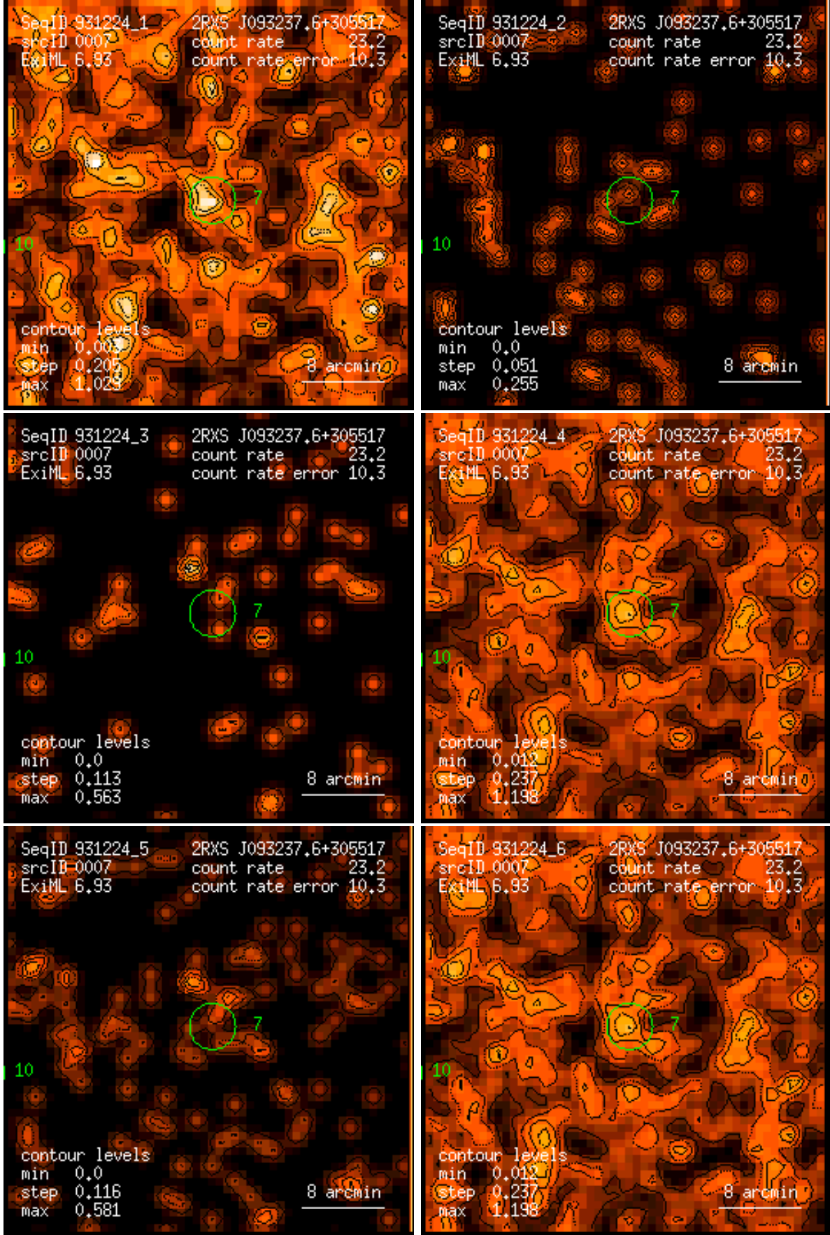
Figure 7: RASS 931224: detection 0007: band rate images, Gaussian filter: (1) PSPC channels 11 – 41, (2) 52 – 90, (3) 91 – 201, (4) 11 – 235, (5) 52 – 201, (6) 11 – 201. Broad band rates in counts/ks. Band rate contour levels in counts/ks/arcmin 2 .
