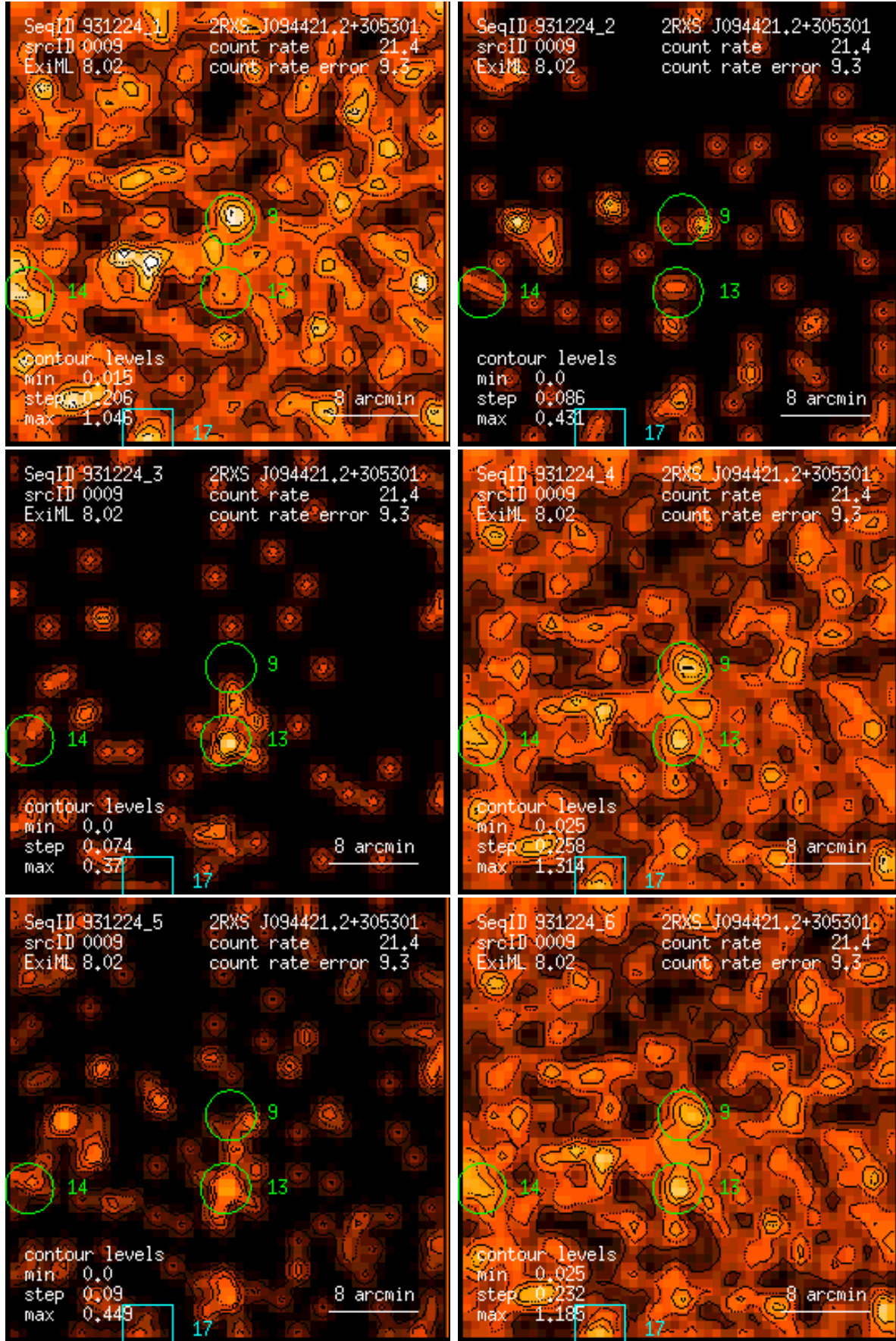
Figure 9: RASS 931224: detection 0009: band rate images, Gaussian filter: (1) PSPC channels 11 – 41, (2) 52 – 90, (3) 91 – 201, (4) 11 – 235, (5) 52 – 201, (6) 11 – 201. Broad band rates in counts/ks. Band rate contour levels in counts/ks/arcmin 2 .
