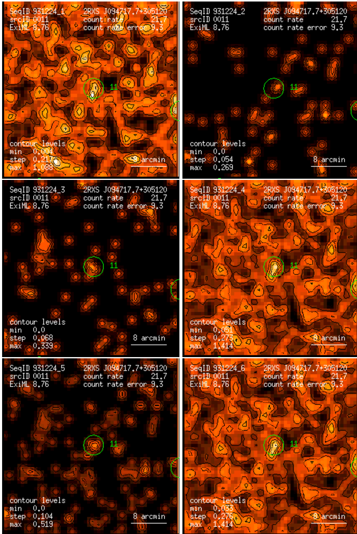
Figure 11: RASS 931224: detection 0011: band rate images, Gaussian filter: (1) PSPC channels 11 – 41, (2) 52 – 90, (3) 91 – 201, (4) 11 – 235, (5) 52 – 201, (6) 11 – 201. Broad band rates in counts/ks. Band rate contour levels in counts/ks/arcmin 2 .
