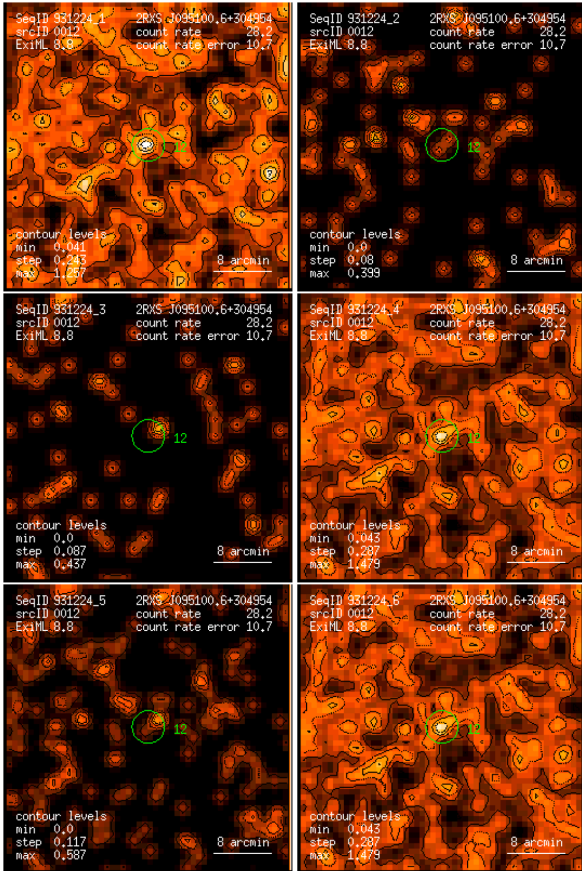
Figure 12: RASS 931224: detection 0012: band rate images, Gaussian filter: (1) PSPC channels 11 – 41, (2) 52 – 90, (3) 91 – 201, (4) 11 – 235, (5) 52 – 201, (6) 11 – 201. Broad band rates in counts/ks. Band rate contour levels in counts/ks/arcmin 2 .
