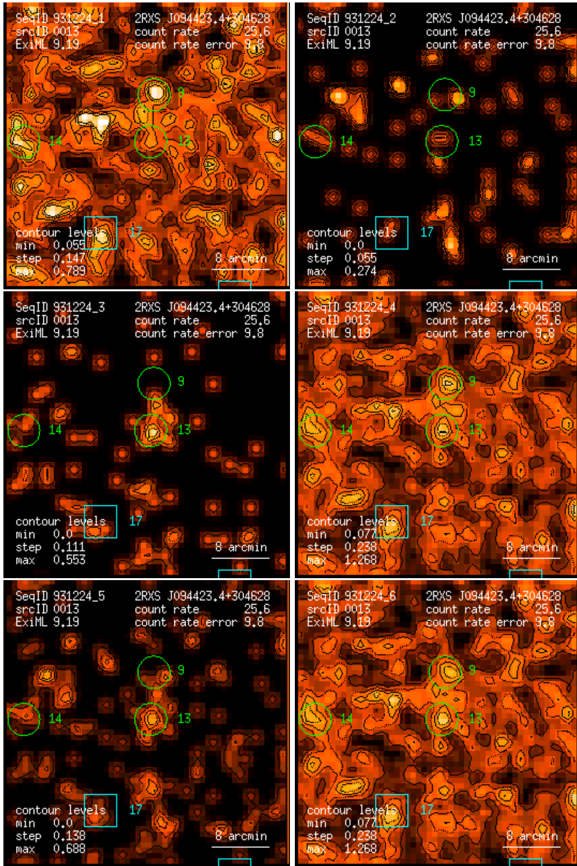
Figure 13: RASS 931224: detection 0013: band rate images, Gaussian filter: (1) PSPC channels 11 – 41, (2) 52 – 90, (3) 91 – 201, (4) 11 – 235, (5) 52 – 201, (6) 11 – 201. Broad band rates in counts/ks. Band rate contour levels in counts/ks/arcmin 2 .
