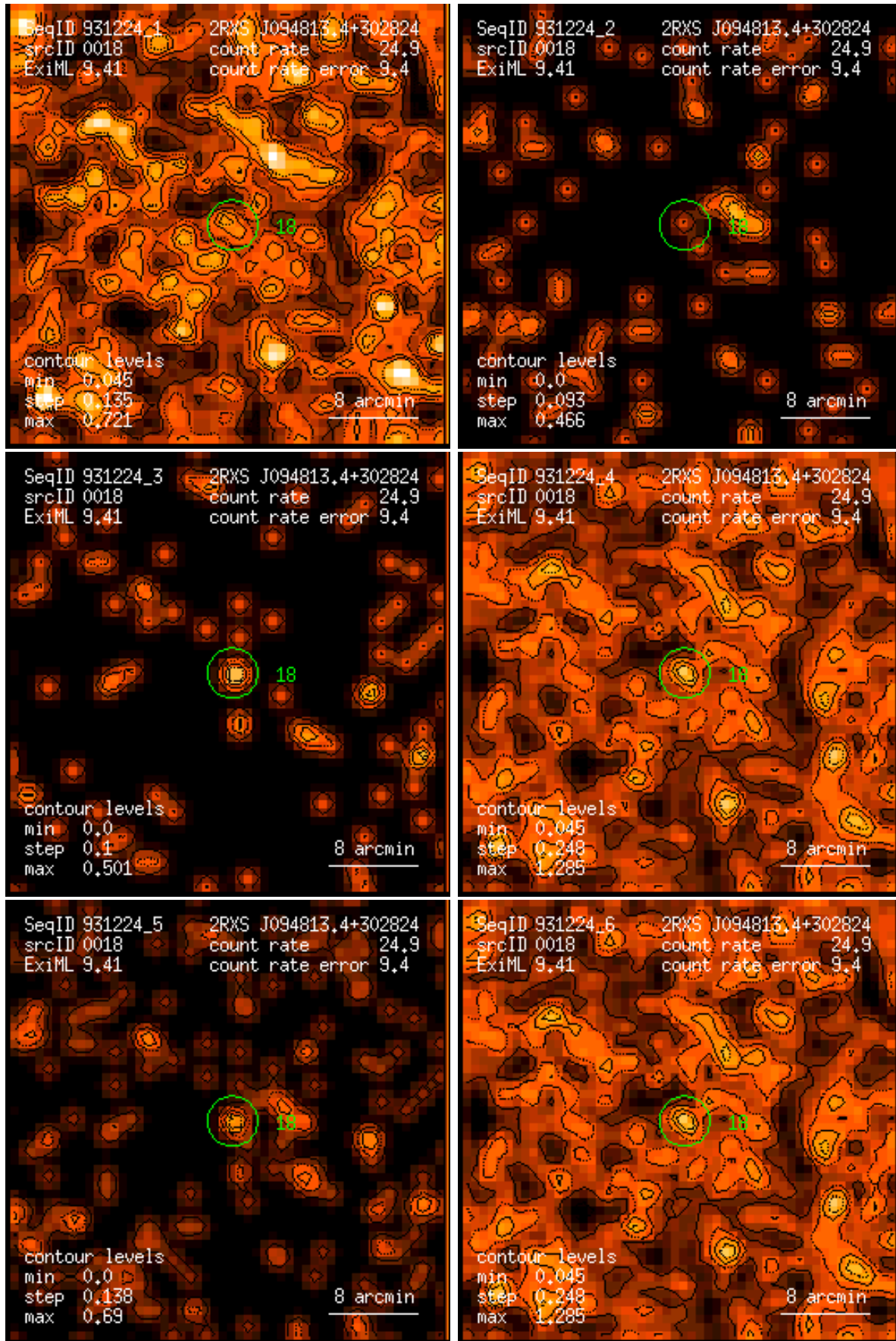
Figure 18: RASS 931224: detection 0018: band rate images, Gaussian filter: (1) PSPC channels 11 – 41, (2) 52 – 90, (3) 91 – 201, (4) 11 – 235, (5) 52 – 201, (6) 11 – 201. Broad band rates in counts/ks. Band rate contour levels in counts/ks/arcmin 2 .
