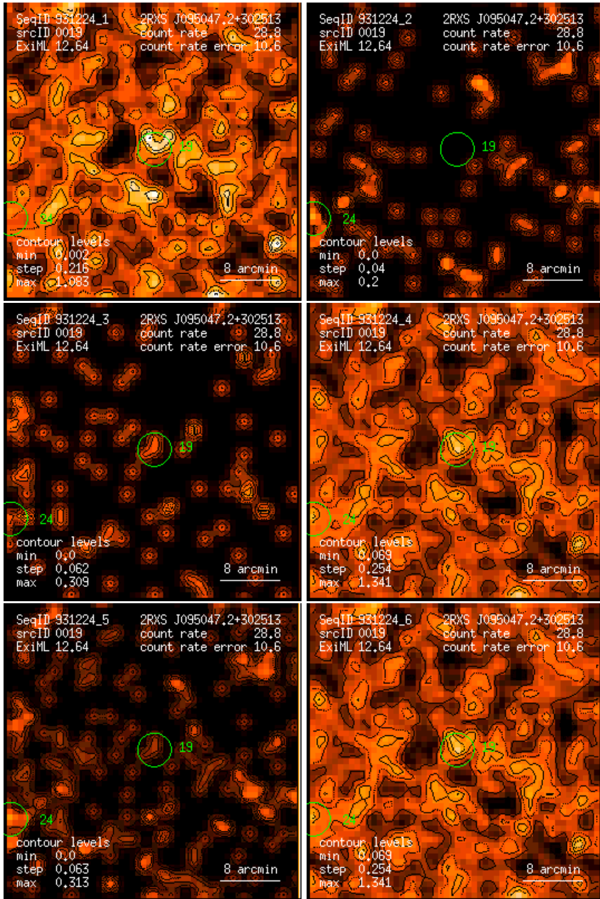
Figure 19: RASS 931224: detection 0019: band rate images, Gaussian filter: (1) PSPC channels 11 – 41, (2) 52 – 90, (3) 91 – 201, (4) 11 – 235, (5) 52 – 201, (6) 11 – 201. Broad band rates in counts/ks. Band rate contour levels in counts/ks/arcmin 2 .
