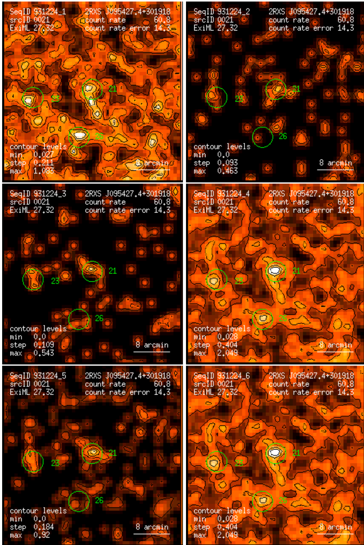
Figure 21: RASS 931224: detection 0021: band rate images, Gaussian filter: (1) PSPC channels 11 – 41, (2) 52 – 90, (3) 91 – 201, (4) 11 – 235, (5) 52 – 201, (6) 11 – 201. Broad band rates in counts/ks. Band rate contour levels in counts/ks/arcmin 2 .
