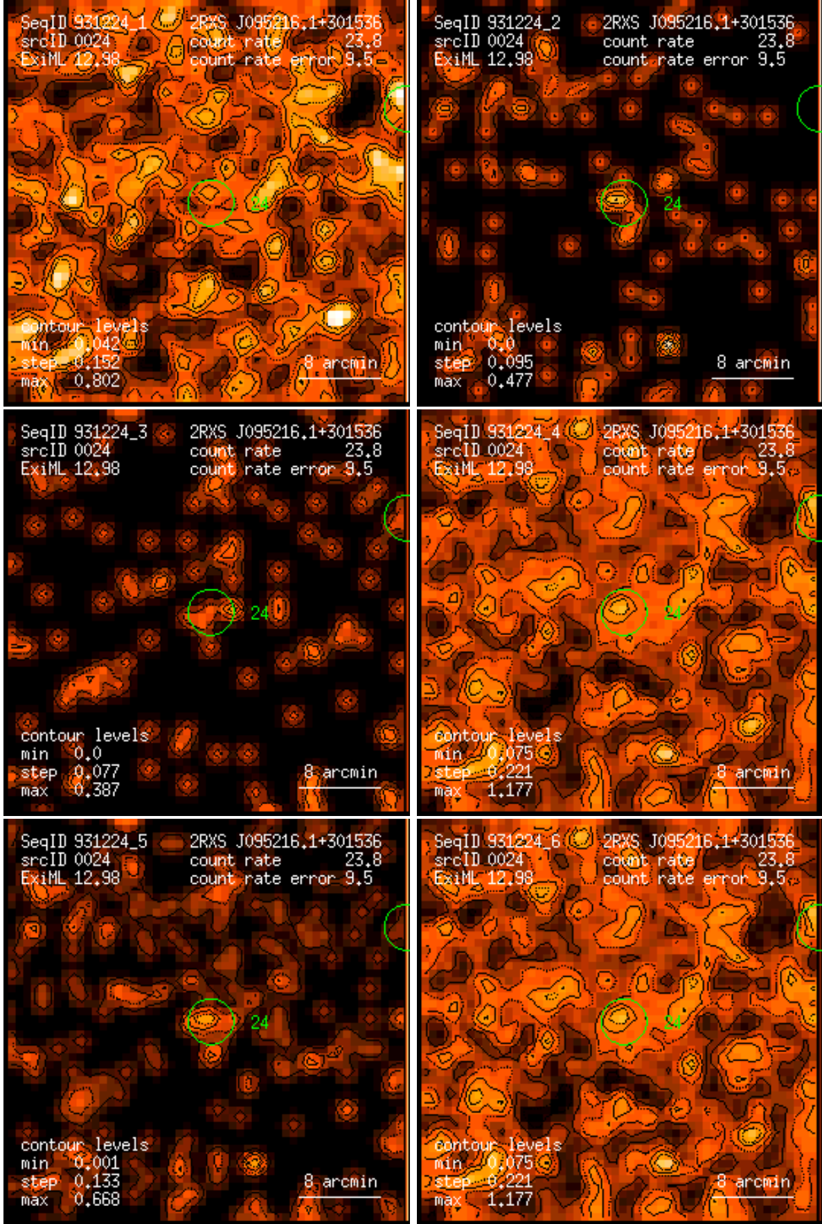
Figure 24: RASS 931224: detection 0024: band rate images, Gaussian filter: (1) PSPC channels 11 – 41, (2) 52 – 90, (3) 91 – 201, (4) 11 – 235, (5) 52 – 201, (6) 11 – 201. Broad band rates in counts/ks. Band rate contour levels in counts/ks/arcmin 2 .
