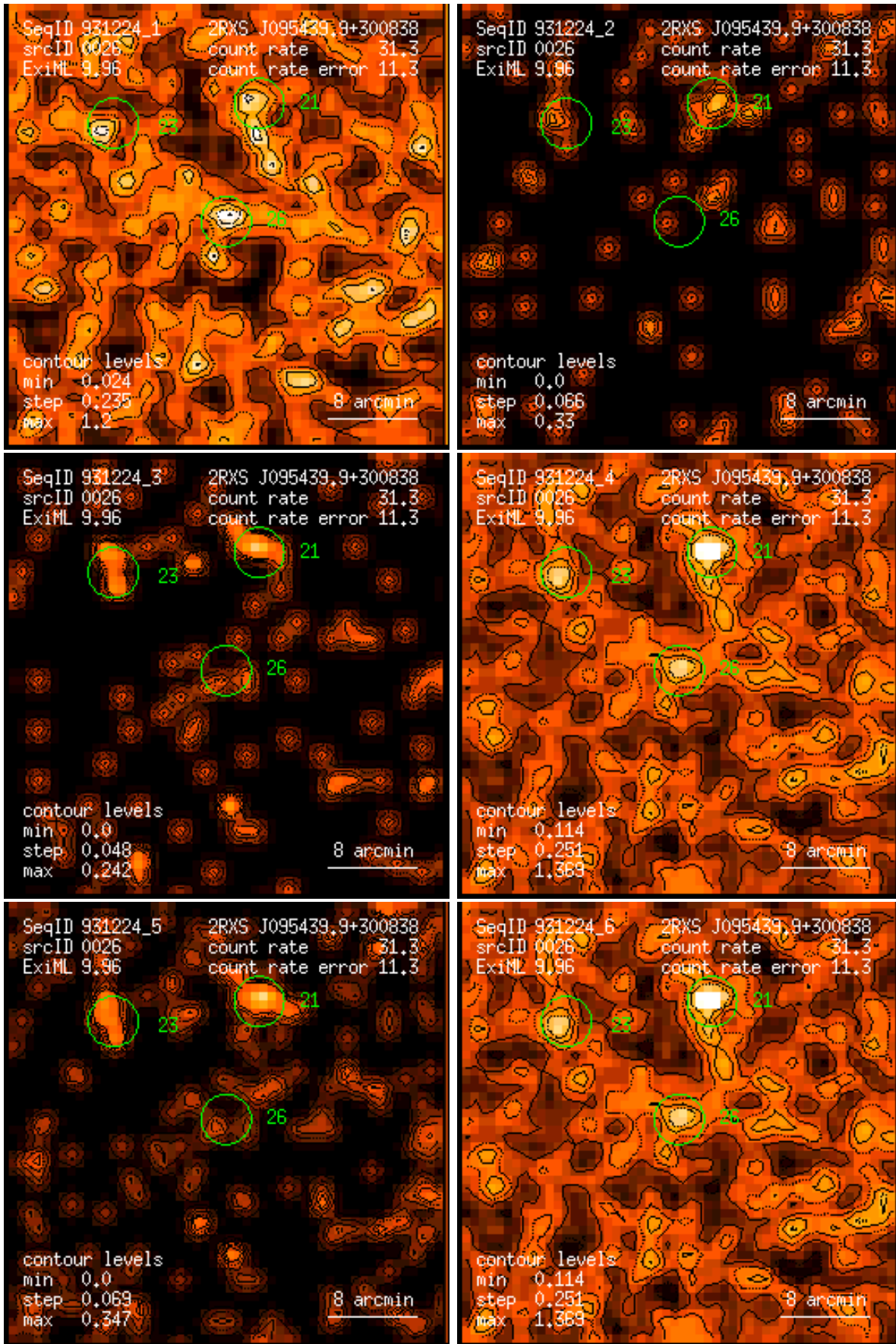
Figure 26: RASS 931224: detection 0026: band rate images, Gaussian filter: (1) PSPC channels 11 – 41, (2) 52 – 90, (3) 91 – 201, (4) 11 – 235, (5) 52 – 201, (6) 11 – 201. Broad band rates in counts/ks. Band rate contour levels in counts/ks/arcmin 2 .
