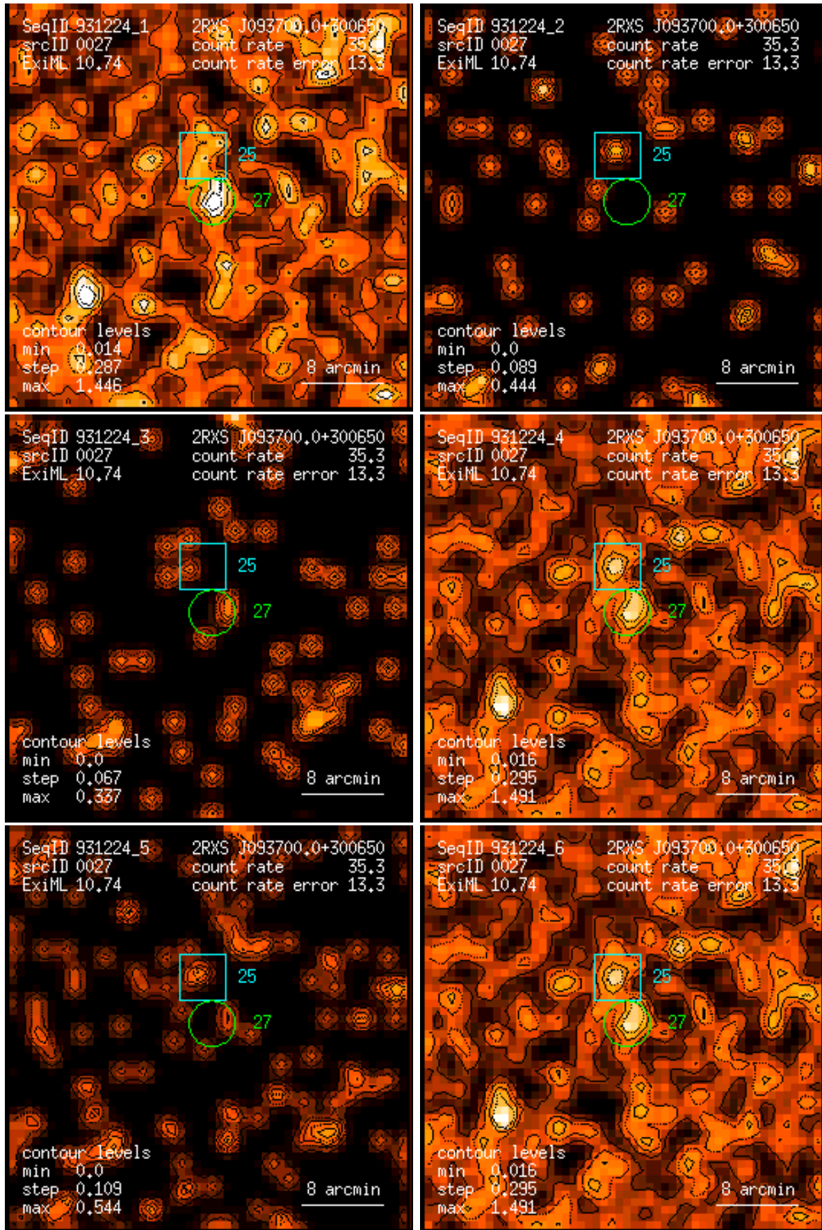
Figure 27: RASS 931224: detection 0027: band rate images, Gaussian filter: (1) PSPC channels 11 – 41, (2) 52 – 90, (3) 91 – 201, (4) 11 – 235, (5) 52 – 201, (6) 11 – 201. Broad band rates in counts/ks. Band rate contour levels in counts/ks/arcmin 2 .
