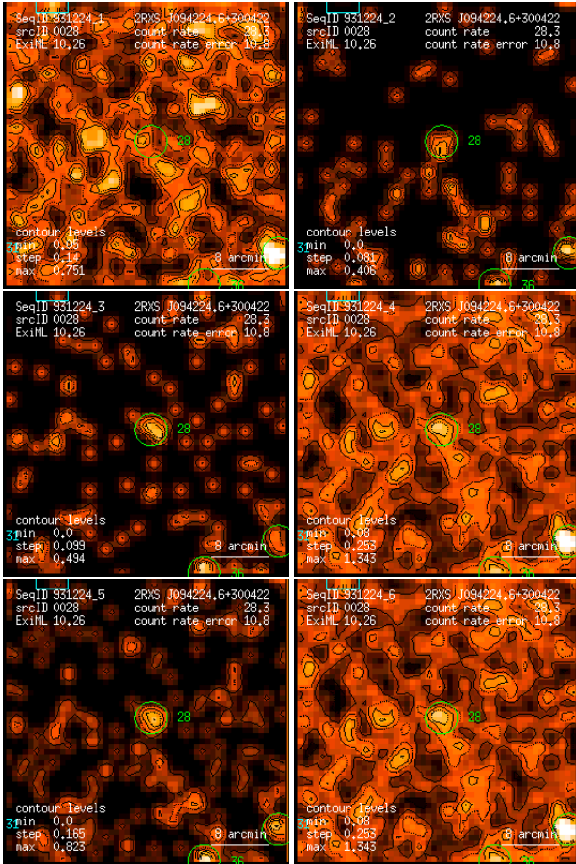
Figure 28: RASS 931224: detection 0028: band rate images, Gaussian filter: (1) PSPC channels 11 – 41, (2) 52 – 90, (3) 91 – 201, (4) 11 – 235, (5) 52 – 201, (6) 11 – 201. Broad band rates in counts/ks. Band rate contour levels in counts/ks/arcmin 2 .
