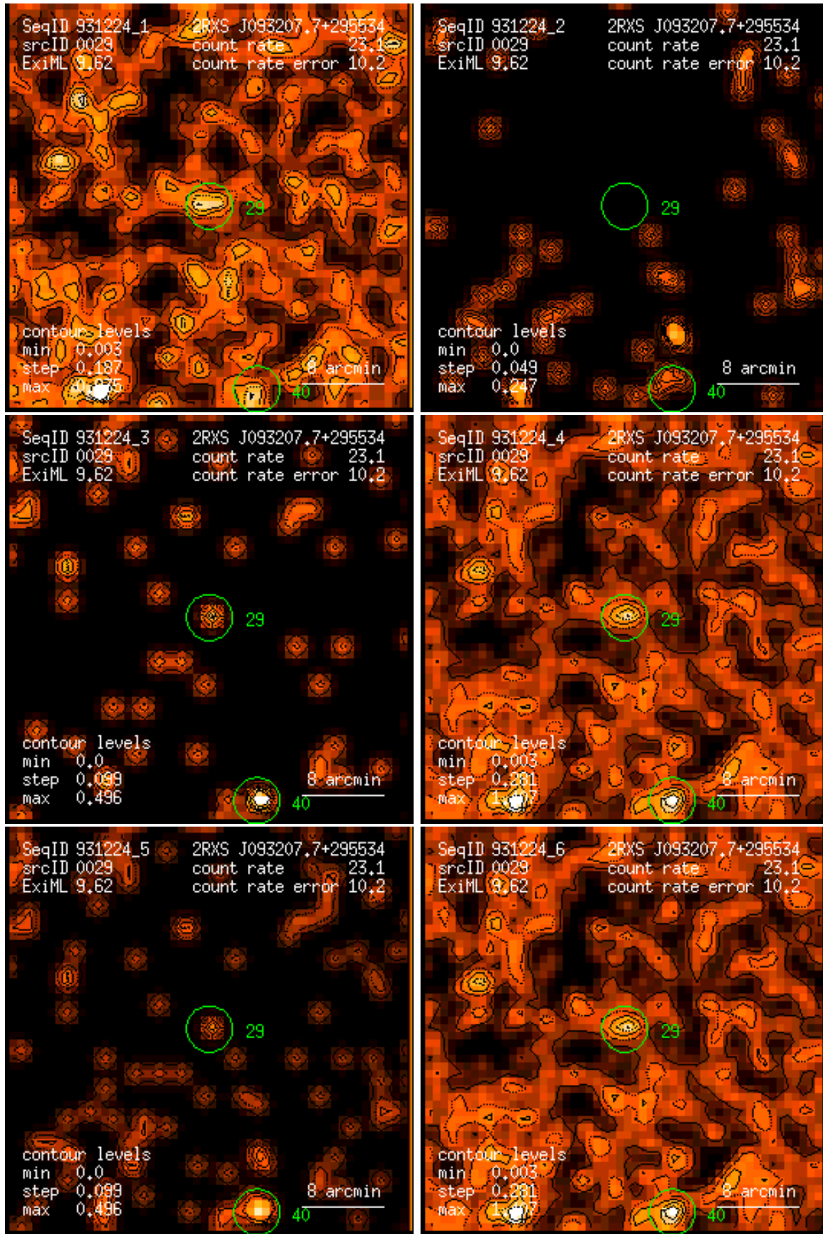
Figure 29: RASS 931224: detection 0029: band rate images, Gaussian filter: (1) PSPC channels 11 – 41, (2) 52 – 90, (3) 91 – 201, (4) 11 – 235, (5) 52 – 201, (6) 11 – 201. Broad band rates in counts/ks. Band rate contour levels in counts/ks/arcmin 2 .
