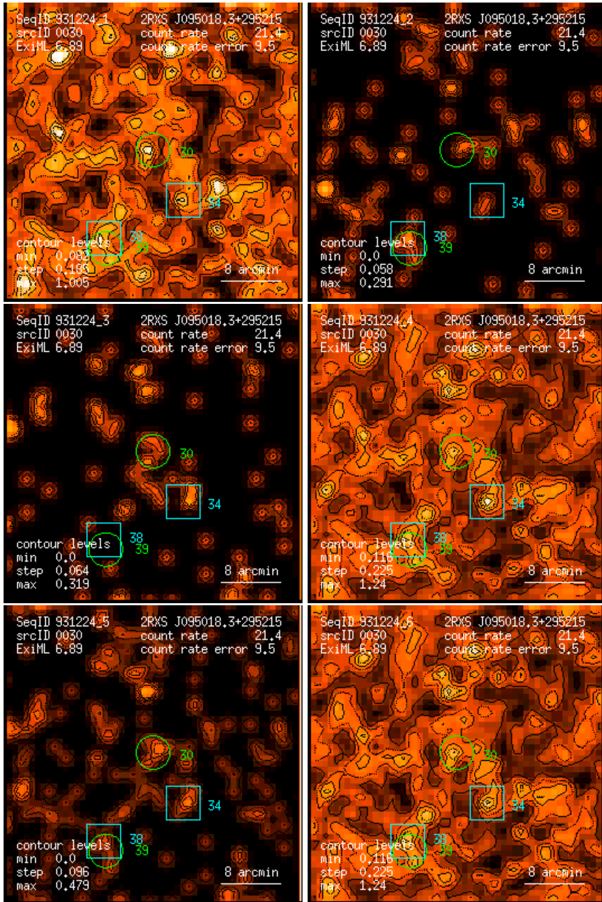
Figure 30: RASS 931224: detection 0030: band rate images, Gaussian filter: (1) PSPC channels 11 – 41, (2) 52 – 90, (3) 91 – 201, (4) 11 – 235, (5) 52 – 201, (6) 11 – 201. Broad band rates in counts/ks. Band rate contour levels in counts/ks/arcmin 2 .
