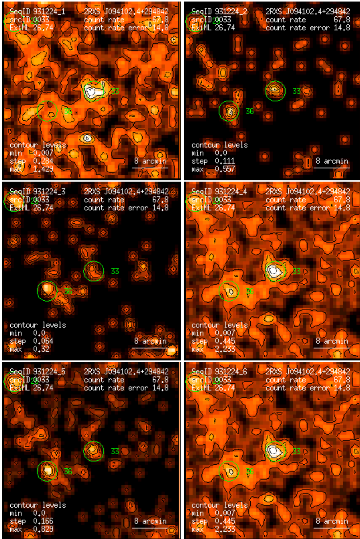
Figure 33: RASS 931224: detection 0033: band rate images, Gaussian filter: (1) PSPC channels 11 – 41, (2) 52 – 90, (3) 91 – 201, (4) 11 – 235, (5) 52 – 201, (6) 11 – 201. Broad band rates in counts/ks. Band rate contour levels in counts/ks/arcmin 2 .
