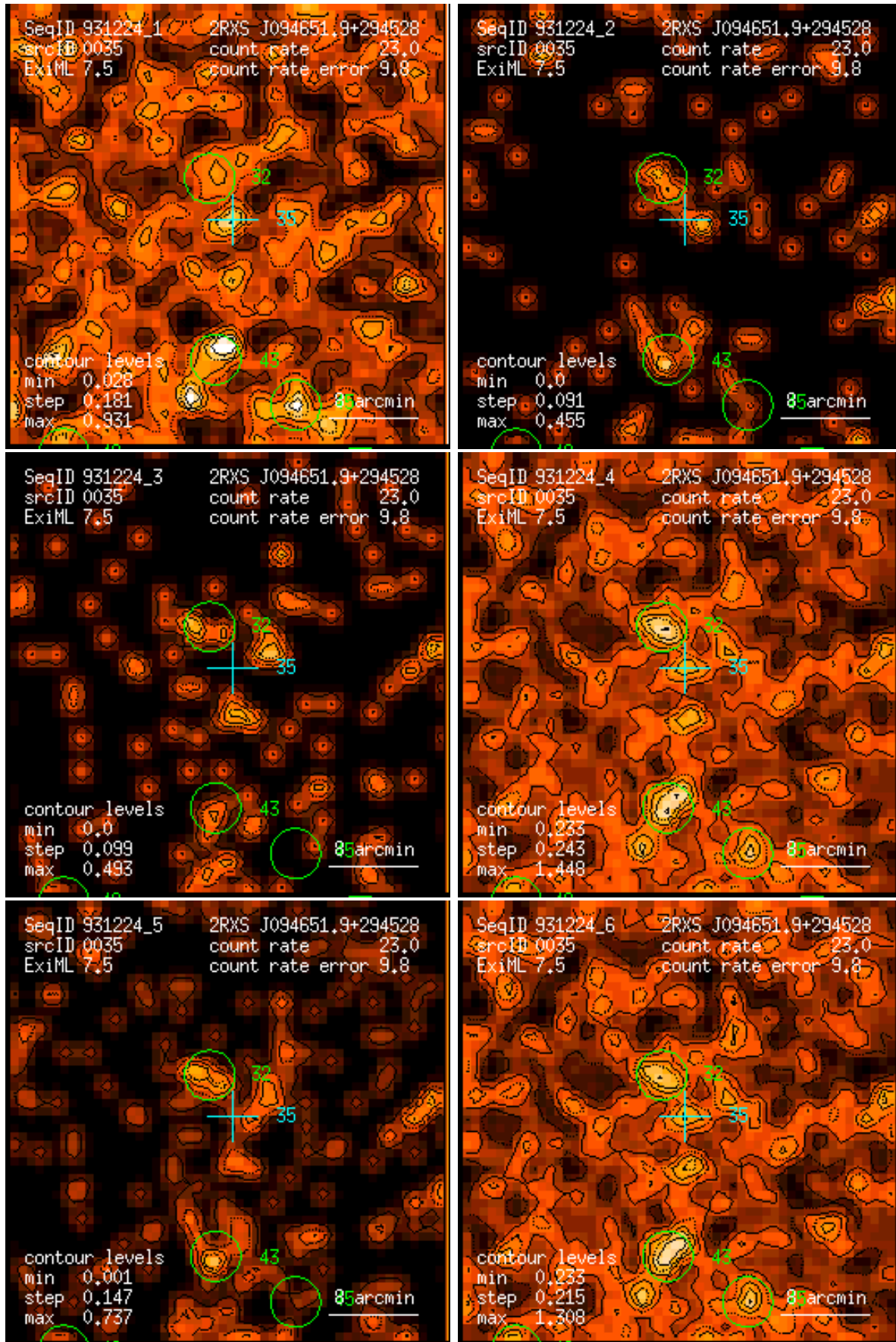
Figure 35: RASS 931224: detection 0035: band rate images, Gaussian filter: (1) PSPC channels 11 – 41, (2) 52 – 90, (3) 91 – 201, (4) 11 – 235, (5) 52 – 201, (6) 11 – 201. Broad band rates in counts/ks. Band rate contour levels in counts/ks/arcmin 2 .
