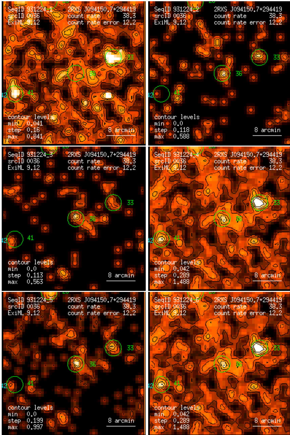
Figure 36: RASS 931224: detection 0036: band rate images, Gaussian filter: (1) PSPC channels 11 – 41, (2) 52 – 90, (3) 91 – 201, (4) 11 – 235, (5) 52 – 201, (6) 11 – 201. Broad band rates in counts/ks. Band rate contour levels in counts/ks/arcmin 2 .
