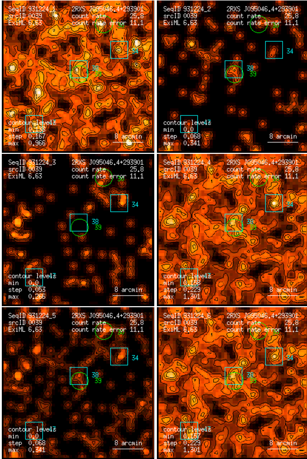
Figure 39: RASS 931224: detection 0039: band rate images, Gaussian filter: (1) PSPC channels 11 – 41, (2) 52 – 90, (3) 91 – 201, (4) 11 – 235, (5) 52 – 201, (6) 11 – 201. Broad band rates in counts/ks. Band rate contour levels in counts/ks/arcmin 2 .
