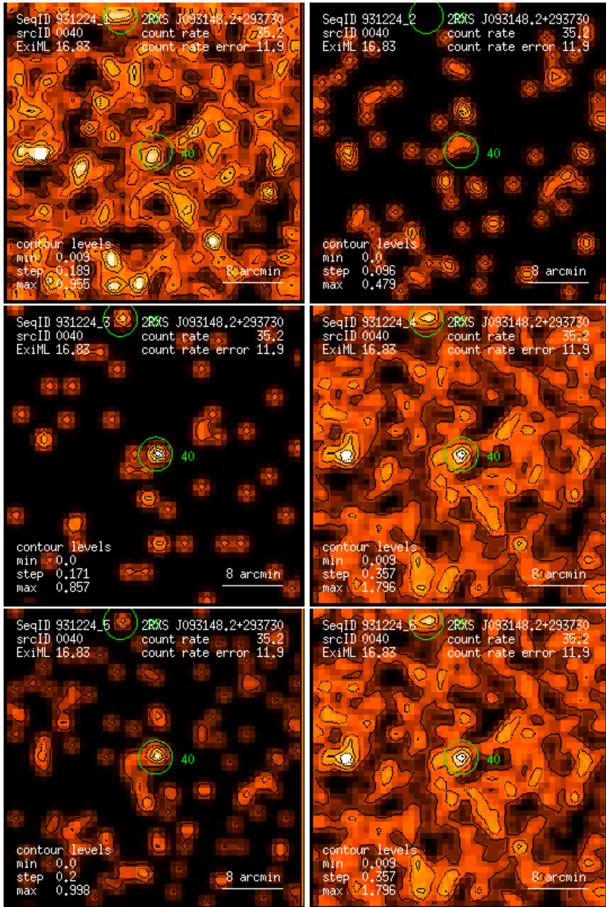
Figure 40: RASS 931224: detection 0040: band rate images, Gaussian filter: (1) PSPC channels 11 – 41, (2) 52 – 90, (3) 91 – 201, (4) 11 – 235, (5) 52 – 201, (6) 11 – 201. Broad band rates in counts/ks. Band rate contour levels in counts/ks/arcmin 2 .
