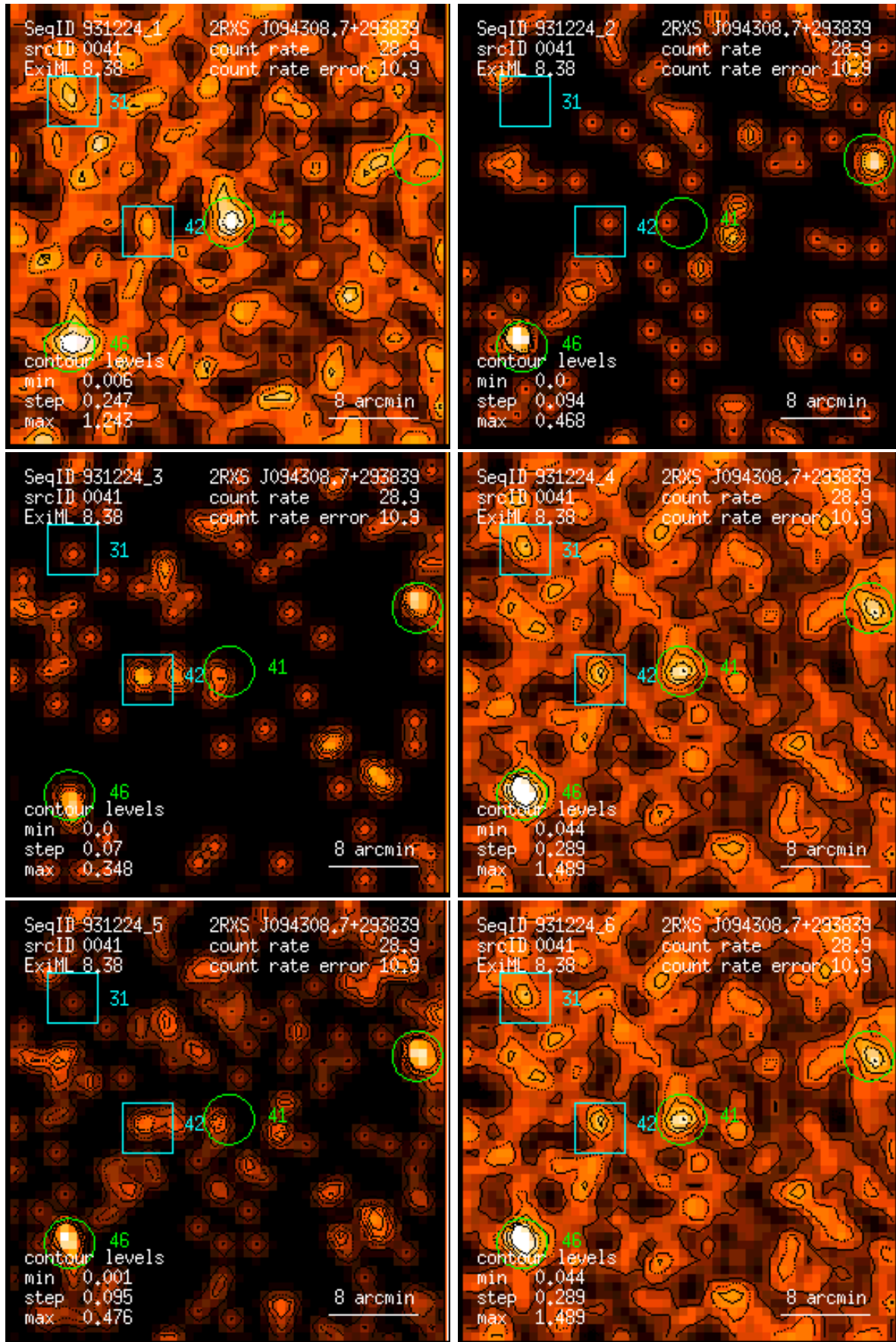
Figure 41: RASS 931224: detection 0041: band rate images, Gaussian filter: (1) PSPC channels 11 – 41, (2) 52 – 90, (3) 91 – 201, (4) 11 – 235, (5) 52 – 201, (6) 11 – 201. Broad band rates in counts/ks. Band rate contour levels in counts/ks/arcmin 2 .
