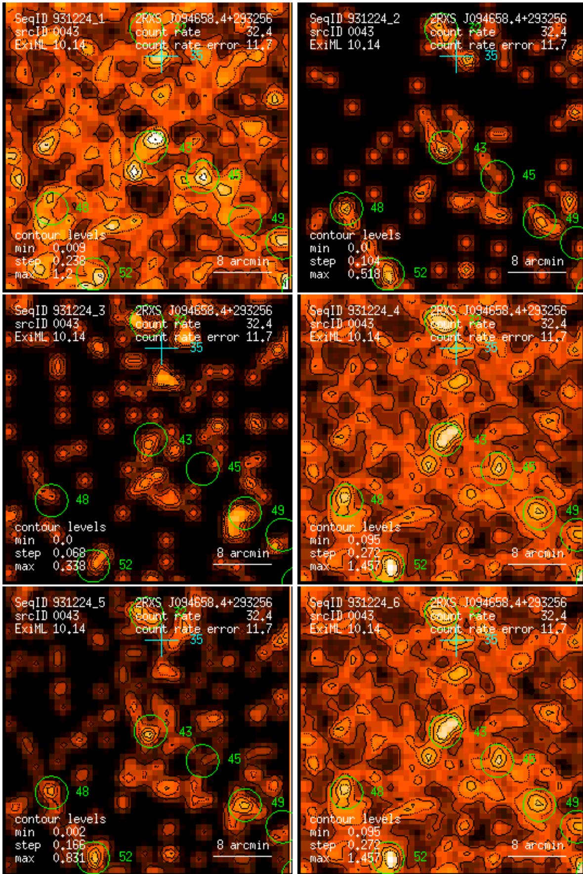
Figure 43: RASS 931224: detection 0043: band rate images, Gaussian filter: (1) PSPC channels 11 – 41, (2) 52 – 90, (3) 91 – 201, (4) 11 – 235, (5) 52 – 201, (6) 11 – 201. Broad band rates in counts/ks. Band rate contour levels in counts/ks/arcmin 2 .
