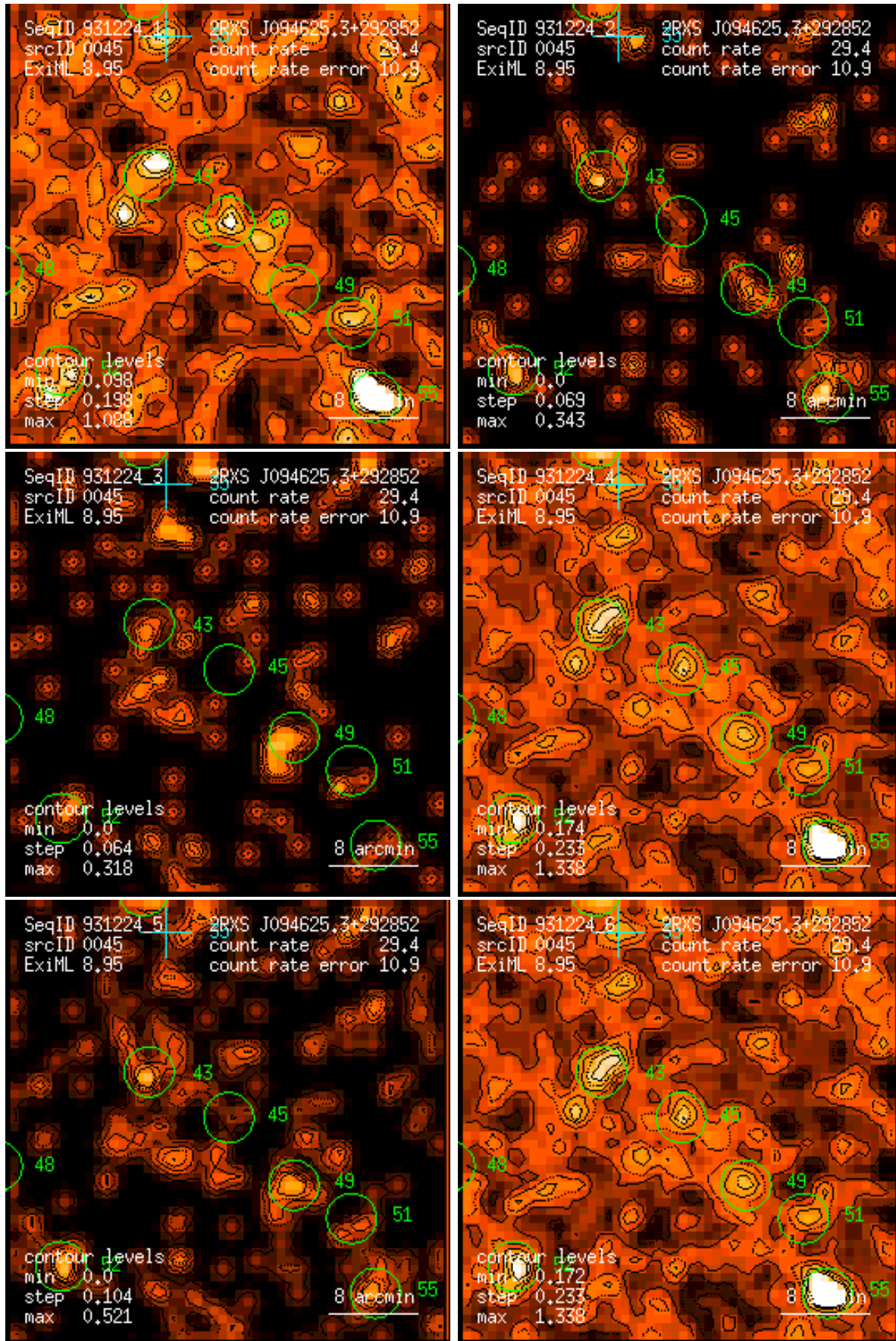
Figure 45: RASS 931224: detection 0045: band rate images, Gaussian filter: (1) PSPC channels 11 – 41, (2) 52 – 90, (3) 91 – 201, (4) 11 – 235, (5) 52 – 201, (6) 11 – 201. Broad band rates in counts/ks. Band rate contour levels in counts/ks/arcmin 2 .
