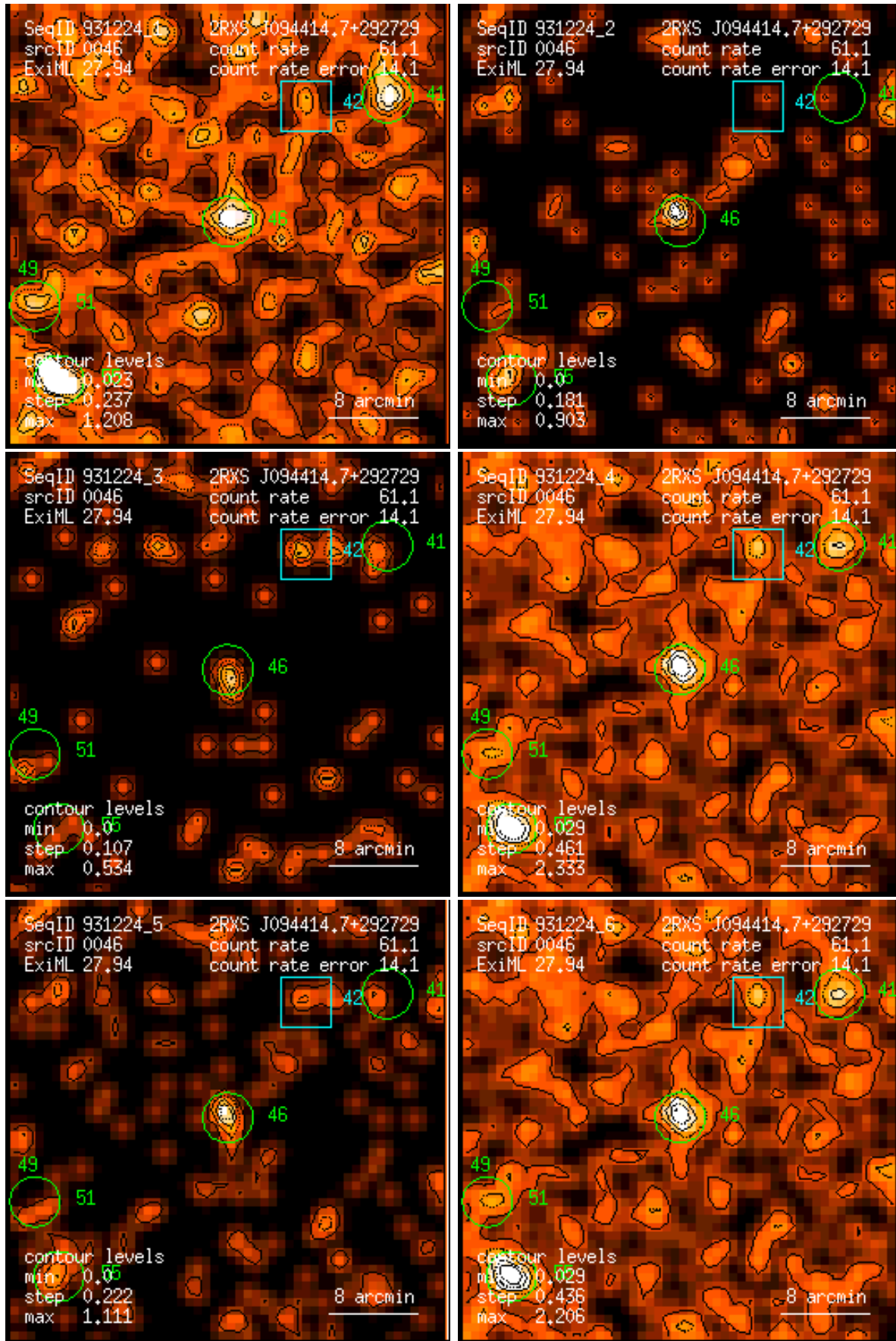
Figure 46: RASS 931224: detection 0046: band rate images, Gaussian filter: (1) PSPC channels 11 – 41, (2) 52 – 90, (3) 91 – 201, (4) 11 – 235, (5) 52 – 201, (6) 11 – 201. Broad band rates in counts/ks. Band rate contour levels in counts/ks/arcmin 2 .
