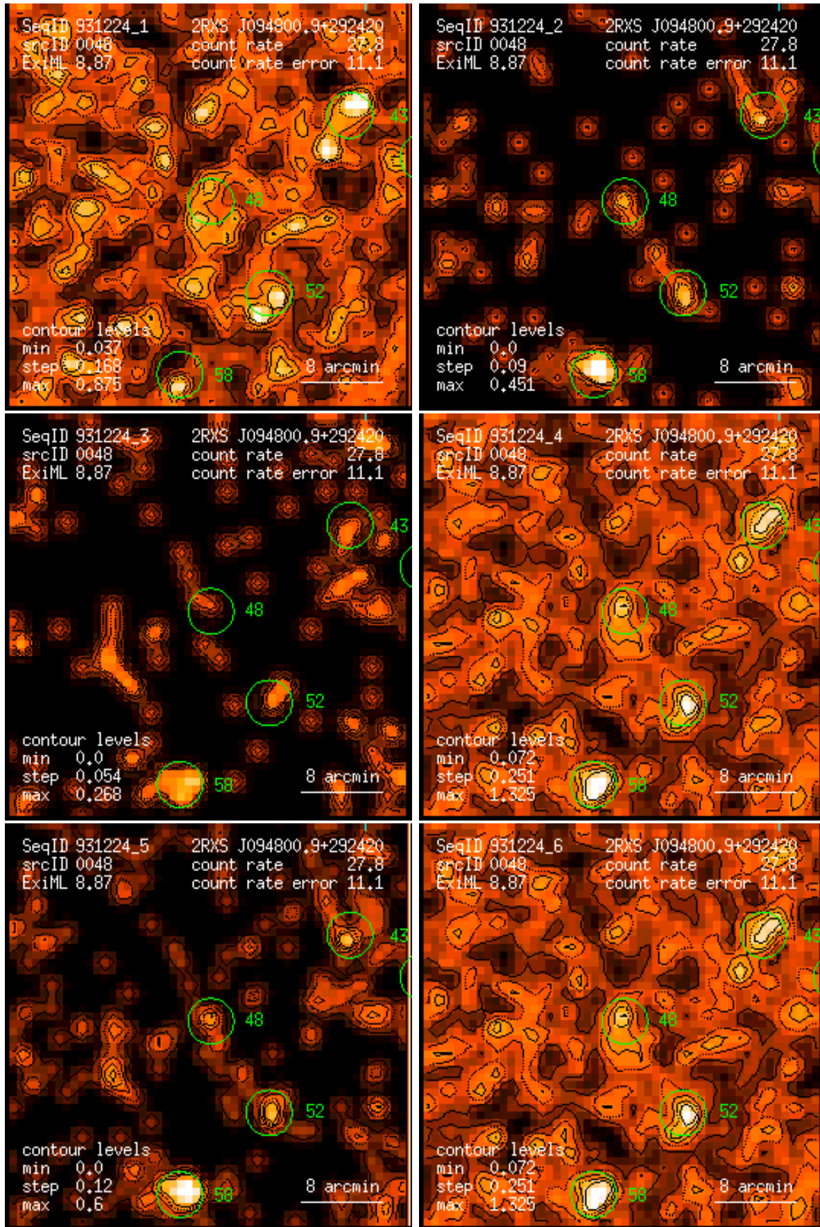
Figure 48: RASS 931224: detection 0048: band rate images, Gaussian filter: (1) PSPC channels 11 – 41, (2) 52 – 90, (3) 91 – 201, (4) 11 – 235, (5) 52 – 201, (6) 11 – 201. Broad band rates in counts/ks. Band rate contour levels in counts/ks/arcmin 2 .
