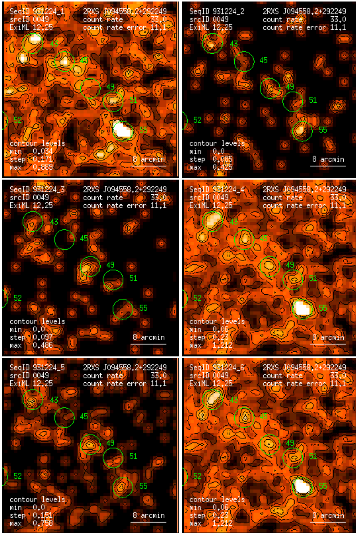
Figure 49: RASS 931224: detection 0049: band rate images, Gaussian filter: (1) PSPC channels 11 – 41, (2) 52 – 90, (3) 91 – 201, (4) 11 – 235, (5) 52 – 201, (6) 11 – 201. Broad band rates in counts/ks. Band rate contour levels in counts/ks/arcmin 2 .
