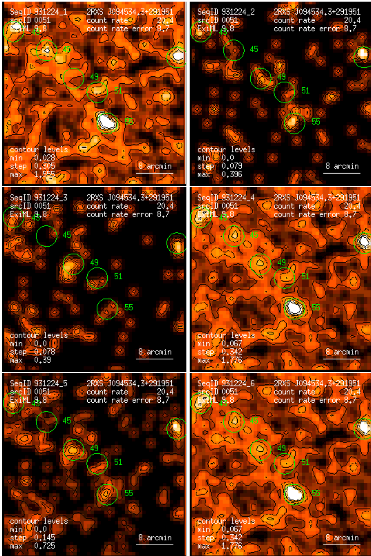
Figure 51: RASS 931224: detection 0051: band rate images, Gaussian filter: (1) PSPC channels 11 – 41, (2) 52 – 90, (3) 91 – 201, (4) 11 – 235, (5) 52 – 201, (6) 11 – 201. Broad band rates in counts/ks. Band rate contour levels in counts/ks/arcmin 2 .
