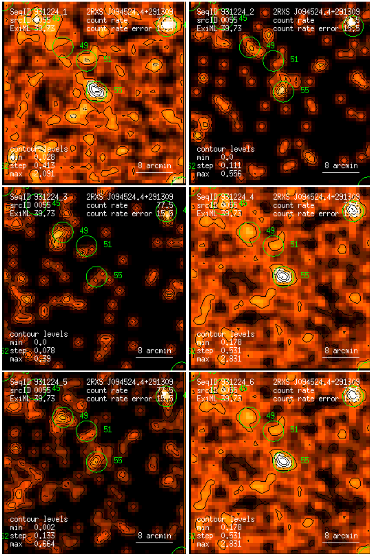
Figure 55: RASS 931224: detection 0055: band rate images, Gaussian filter: (1) PSPC channels 11 – 41, (2) 52 – 90, (3) 91 – 201, (4) 11 – 235, (5) 52 – 201, (6) 11 – 201. Broad band rates in counts/ks. Band rate contour levels in counts/ks/arcmin 2 .
