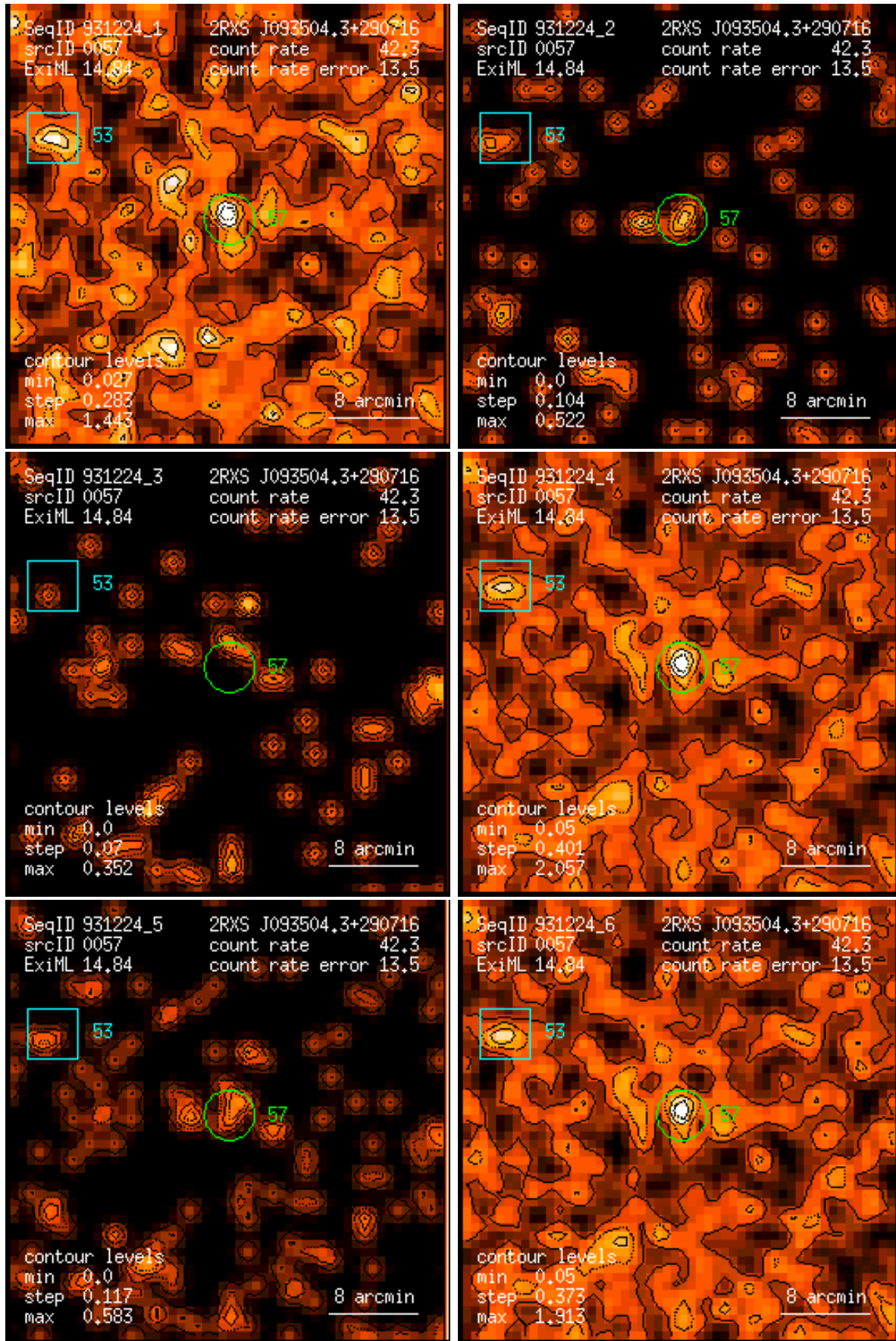
Figure 57: RASS 931224: detection 0057: band rate images, Gaussian filter: (1) PSPC channels 11 – 41, (2) 52 – 90, (3) 91 – 201, (4) 11 – 235, (5) 52 – 201, (6) 11 – 201. Broad band rates in counts/ks. Band rate contour levels in counts/ks/arcmin 2 .
