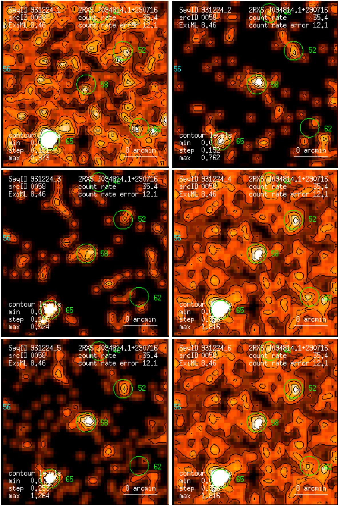
Figure 58: RASS 931224: detection 0058: band rate images, Gaussian filter: (1) PSPC channels 11 – 41, (2) 52 – 90, (3) 91 – 201, (4) 11 – 235, (5) 52 – 201, (6) 11 – 201. Broad band rates in counts/ks. Band rate contour levels in counts/ks/arcmin 2 .
