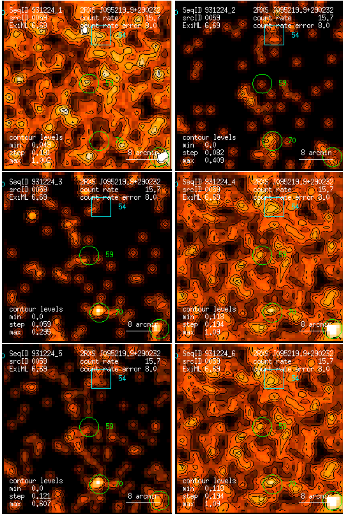
Figure 59: RASS 931224: detection 0059: band rate images, Gaussian filter: (1) PSPC channels 11 – 41, (2) 52 – 90, (3) 91 – 201, (4) 11 – 235, (5) 52 – 201, (6) 11 – 201. Broad band rates in counts/ks. Band rate contour levels in counts/ks/arcmin 2 .
