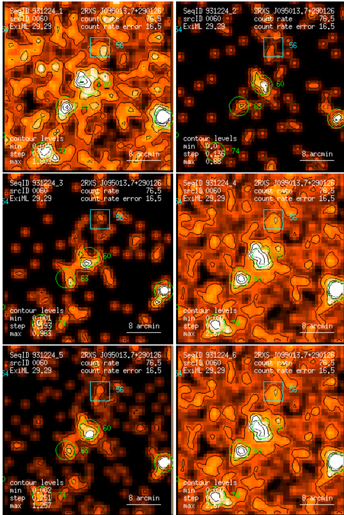
Figure 60: RASS 931224: detection 0060: band rate images, Gaussian filter: (1) PSPC channels 11 – 41, (2) 52 – 90, (3) 91 – 201, (4) 11 – 235, (5) 52 – 201, (6) 11 – 201. Broad band rates in counts/ks. Band rate contour levels in counts/ks/arcmin 2 .
