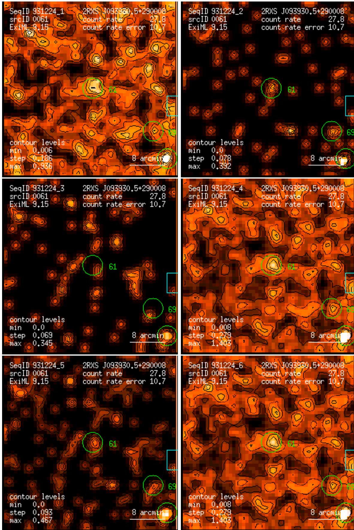
Figure 61: RASS 931224: detection 0061: band rate images, Gaussian filter: (1) PSPC channels 11 – 41, (2) 52 – 90, (3) 91 – 201, (4) 11 – 235, (5) 52 – 201, (6) 11 – 201. Broad band rates in counts/ks. Band rate contour levels in counts/ks/arcmin 2 .
