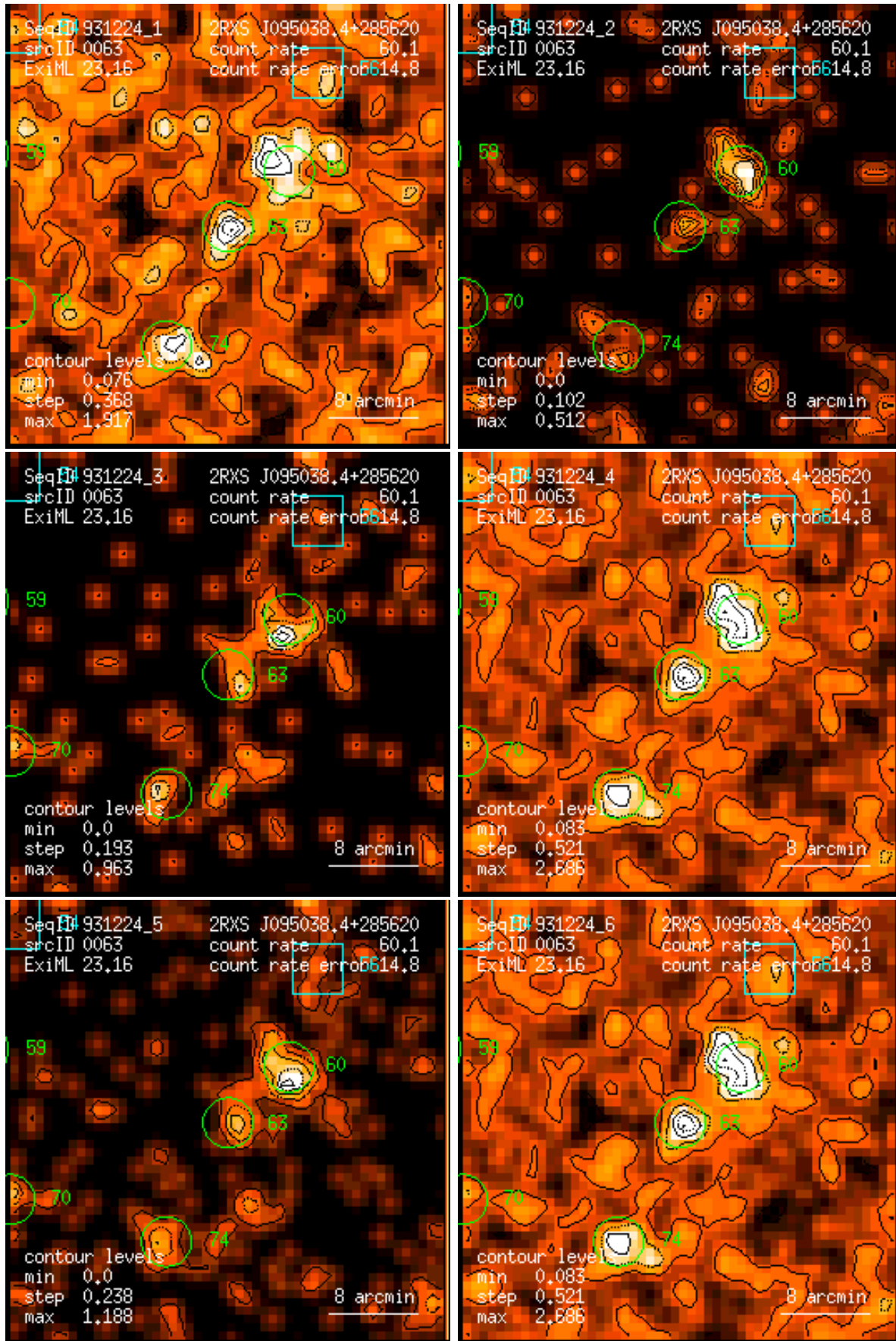
Figure 63: RASS 931224: detection 0063: band rate images, Gaussian filter: (1) PSPC channels 11 – 41, (2) 52 – 90, (3) 91 – 201, (4) 11 – 235, (5) 52 – 201, (6) 11 – 201. Broad band rates in counts/ks. Band rate contour levels in counts/ks/arcmin 2 .
