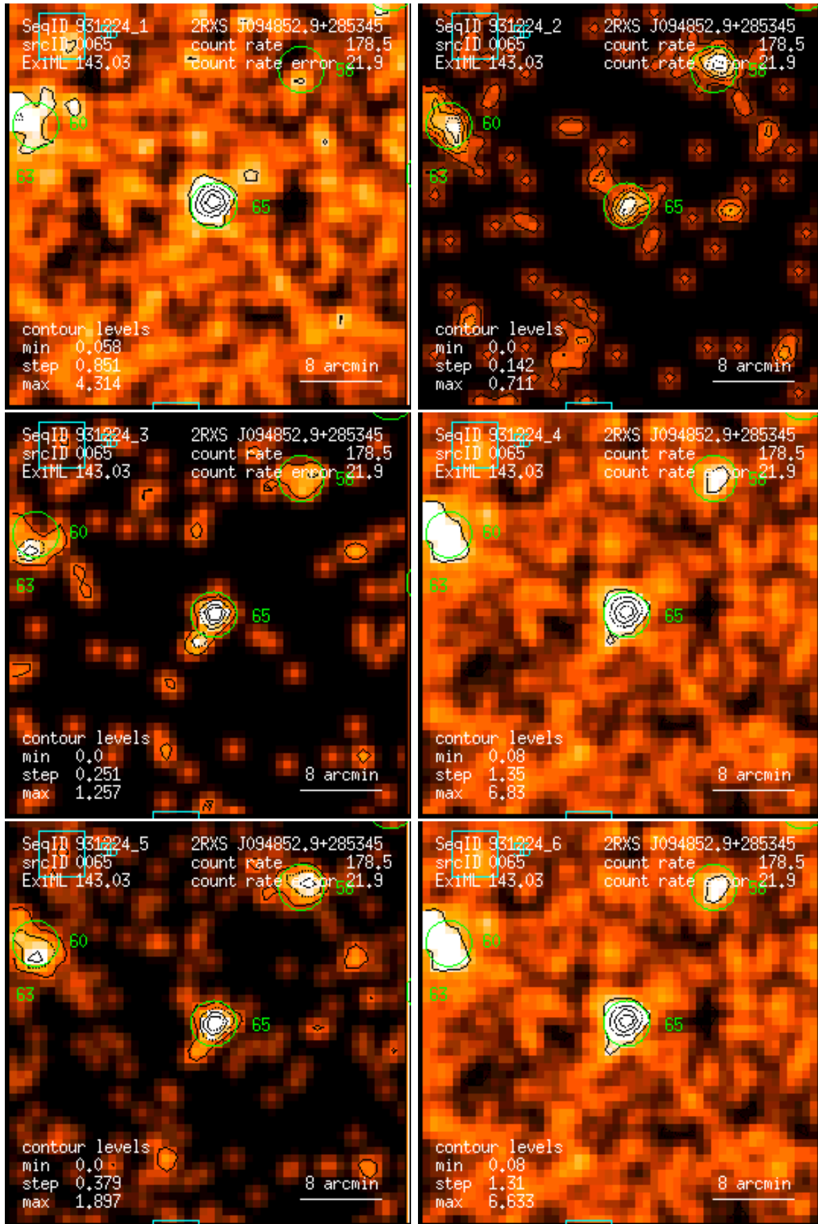
Figure 65: RASS 931224: detection 0065: band rate images, Gaussian filter: (1) PSPC channels 11 – 41, (2) 52 – 90, (3) 91 – 201, (4) 11 – 235, (5) 52 – 201, (6) 11 – 201. Broad band rates in counts/ks. Band rate contour levels in counts/ks/arcmin 2 .
