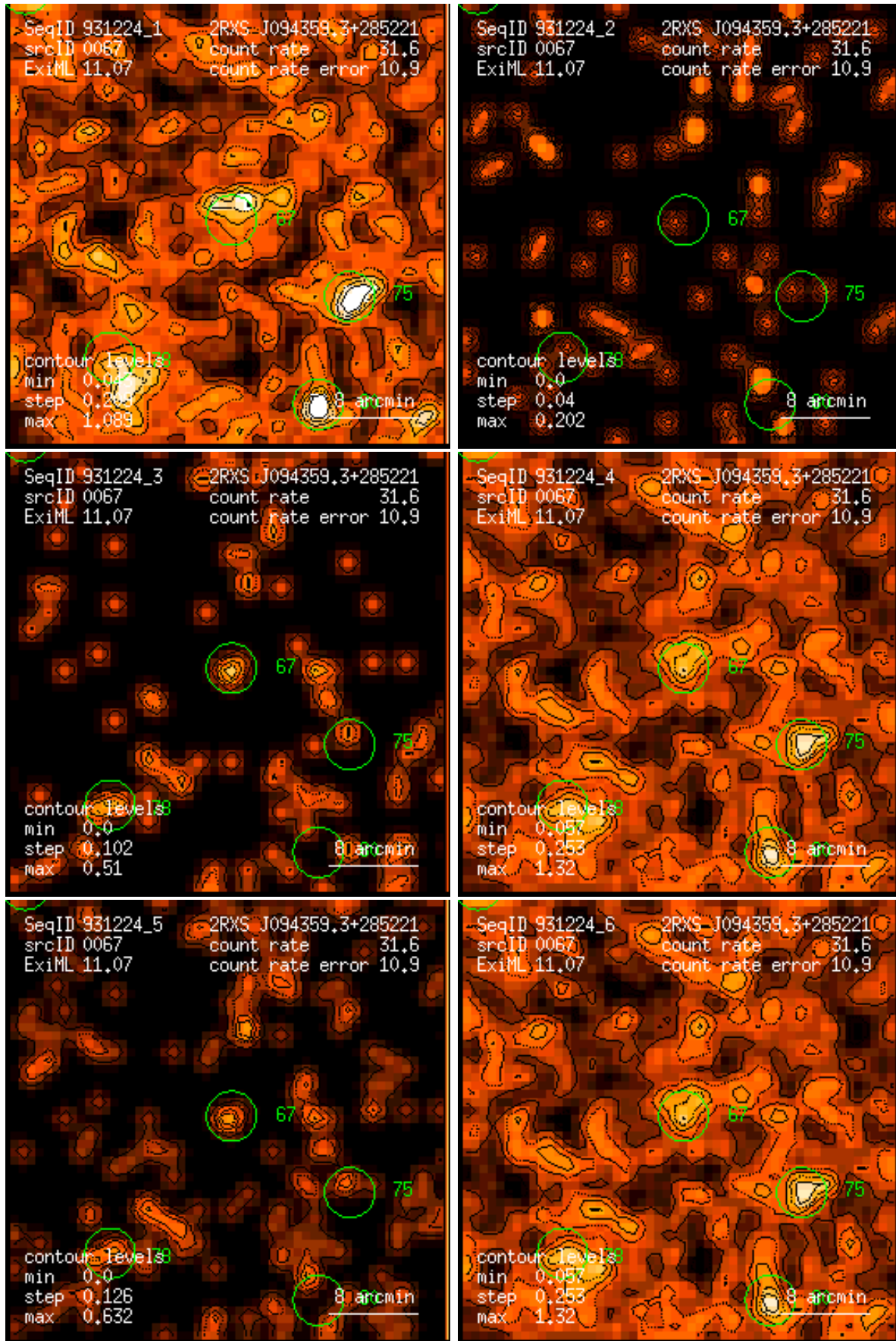
Figure 67: RASS 931224: detection 0067: band rate images, Gaussian filter: (1) PSPC channels 11 – 41, (2) 52 – 90, (3) 91 – 201, (4) 11 – 235, (5) 52 – 201, (6) 11 – 201. Broad band rates in counts/ks. Band rate contour levels in counts/ks/arcmin 2 .
