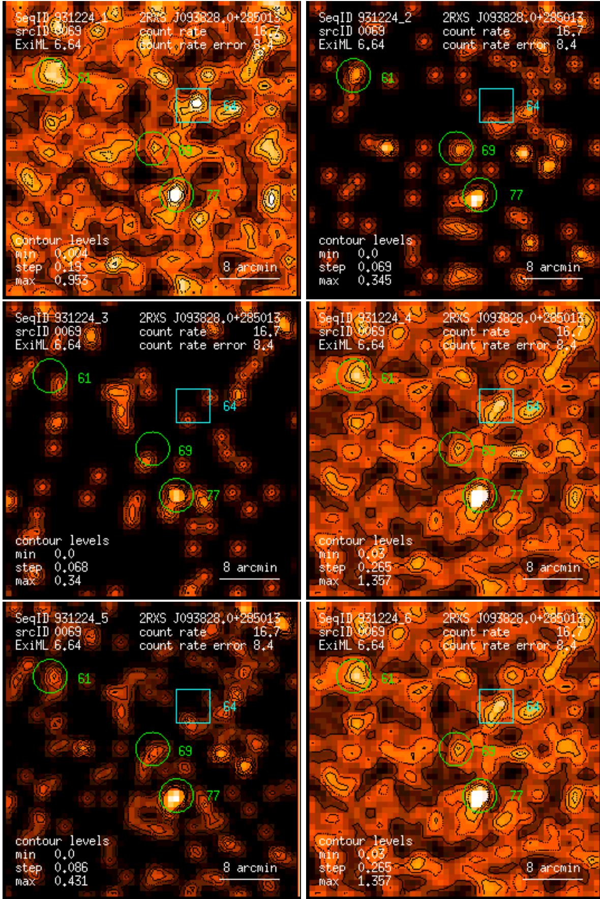
Figure 69: RASS 931224: detection 0069: band rate images, Gaussian filter: (1) PSPC channels 11 – 41, (2) 52 – 90, (3) 91 – 201, (4) 11 – 235, (5) 52 – 201, (6) 11 – 201. Broad band rates in counts/ks. Band rate contour levels in counts/ks/arcmin 2 .
