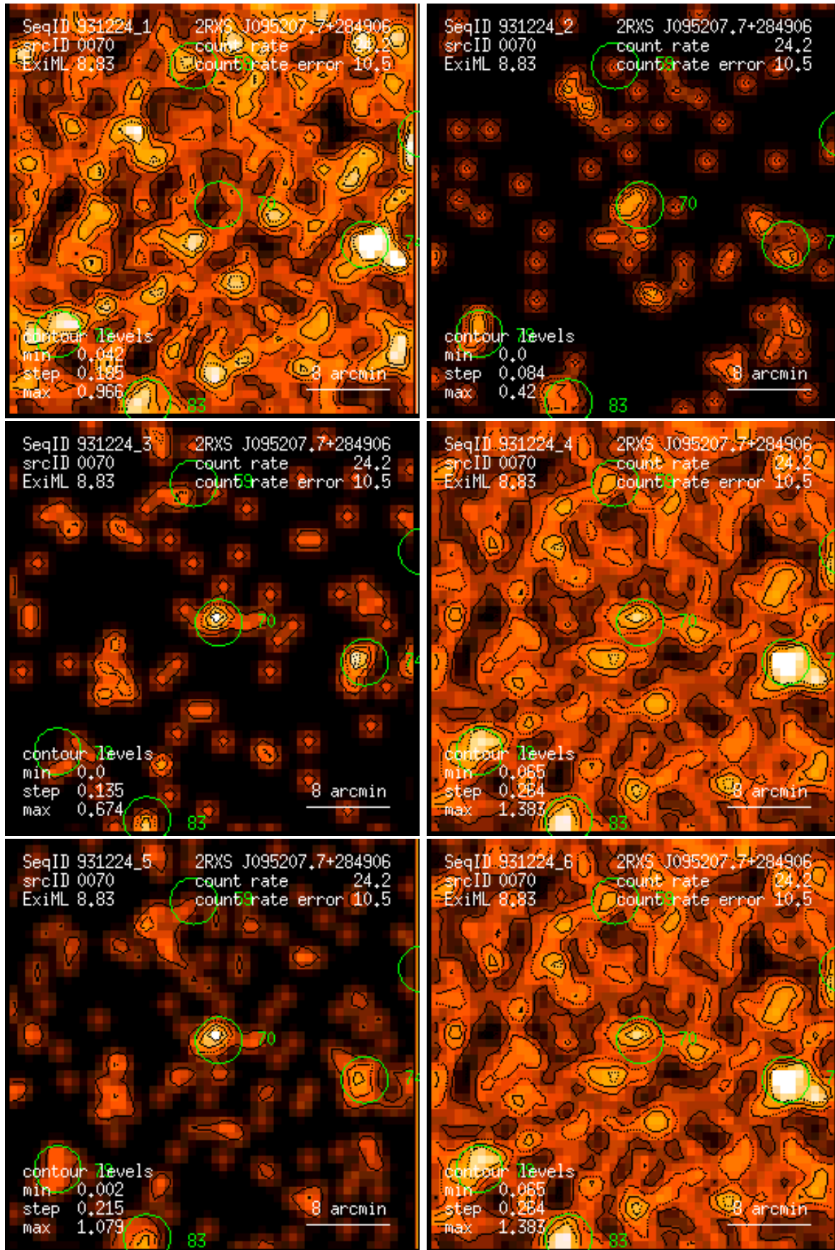
Figure 70: RASS 931224: detection 0070: band rate images, Gaussian filter: (1) PSPC channels 11 – 41, (2) 52 – 90, (3) 91 – 201, (4) 11 – 235, (5) 52 – 201, (6) 11 – 201. Broad band rates in counts/ks. Band rate contour levels in counts/ks/arcmin 2 .
