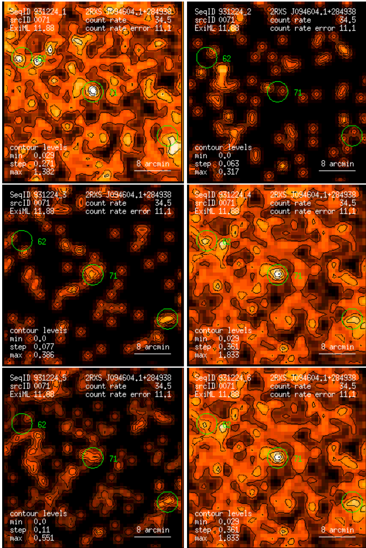
Figure 71: RASS 931224: detection 0071: band rate images, Gaussian filter: (1) PSPC channels 11 – 41, (2) 52 – 90, (3) 91 – 201, (4) 11 – 235, (5) 52 – 201, (6) 11 – 201. Broad band rates in counts/ks. Band rate contour levels in counts/ks/arcmin 2 .
