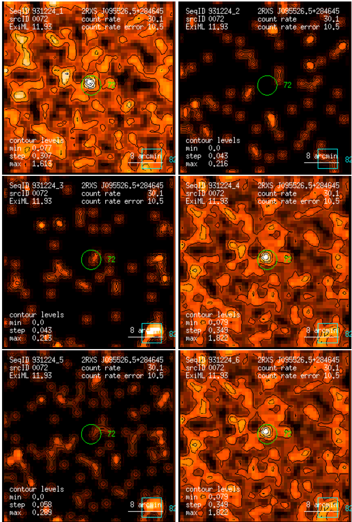
Figure 72: RASS 931224: detection 0072: band rate images, Gaussian filter: (1) PSPC channels 11 – 41, (2) 52 – 90, (3) 91 – 201, (4) 11 – 235, (5) 52 – 201, (6) 11 – 201. Broad band rates in counts/ks. Band rate contour levels in counts/ks/arcmin 2 .
