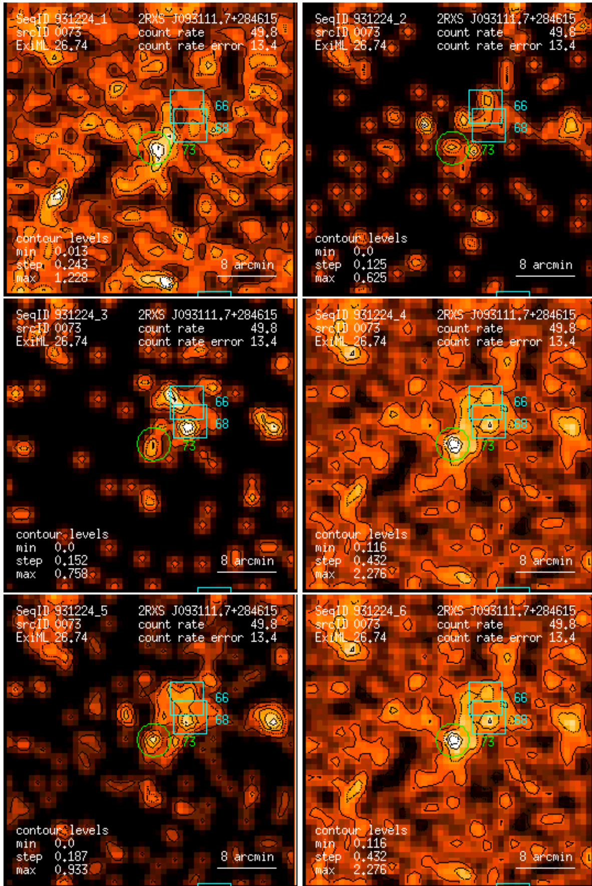
Figure 73: RASS 931224: detection 0073: band rate images, Gaussian filter: (1) PSPC channels 11 – 41, (2) 52 – 90, (3) 91 – 201, (4) 11 – 235, (5) 52 – 201, (6) 11 – 201. Broad band rates in counts/ks. Band rate contour levels in counts/ks/arcmin 2 .
