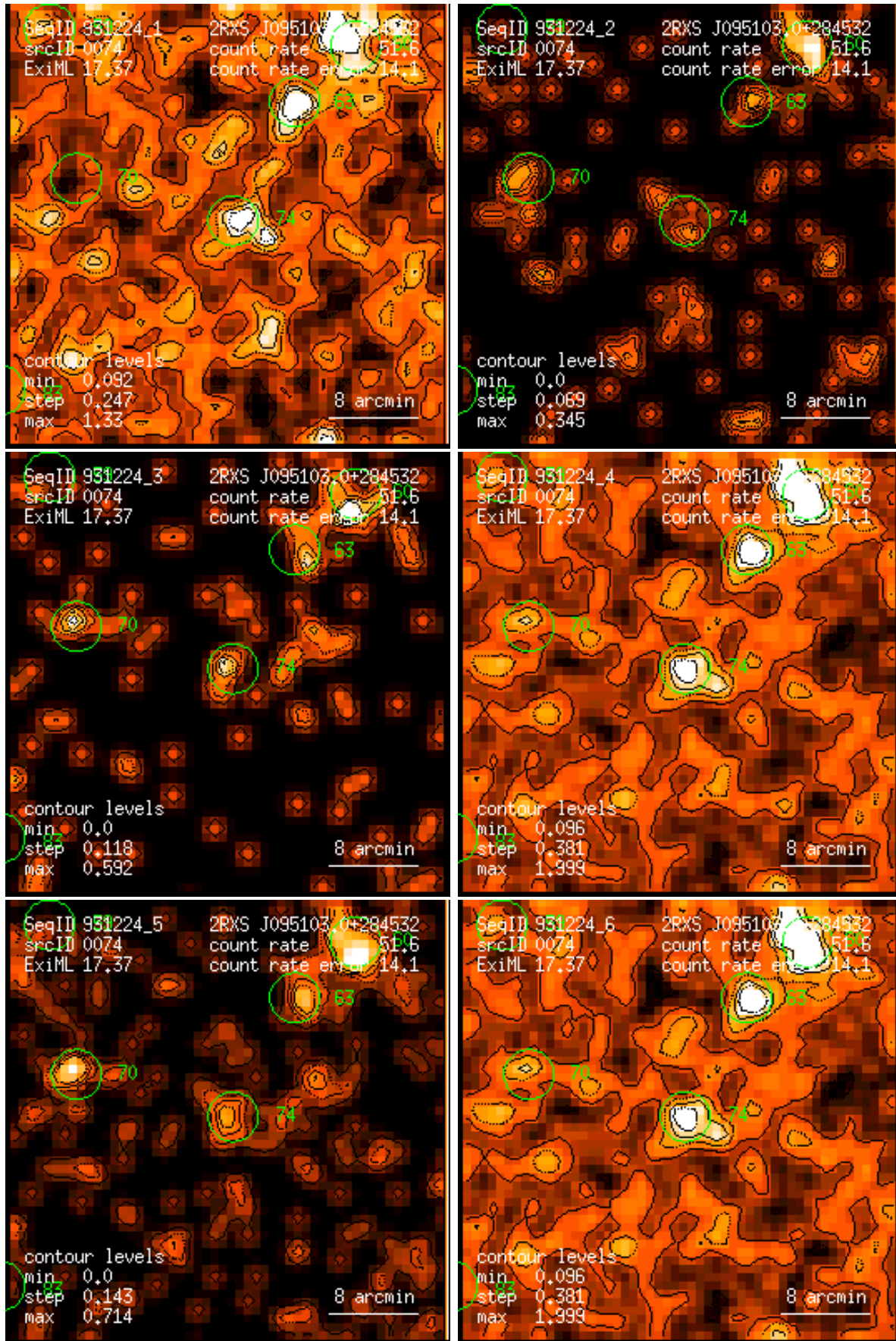
Figure 74: RASS 931224: detection 0074: band rate images, Gaussian filter: (1) PSPC channels 11 – 41, (2) 52 – 90, (3) 91 – 201, (4) 11 – 235, (5) 52 – 201, (6) 11 – 201. Broad band rates in counts/ks. Band rate contour levels in counts/ks/arcmin 2 .
