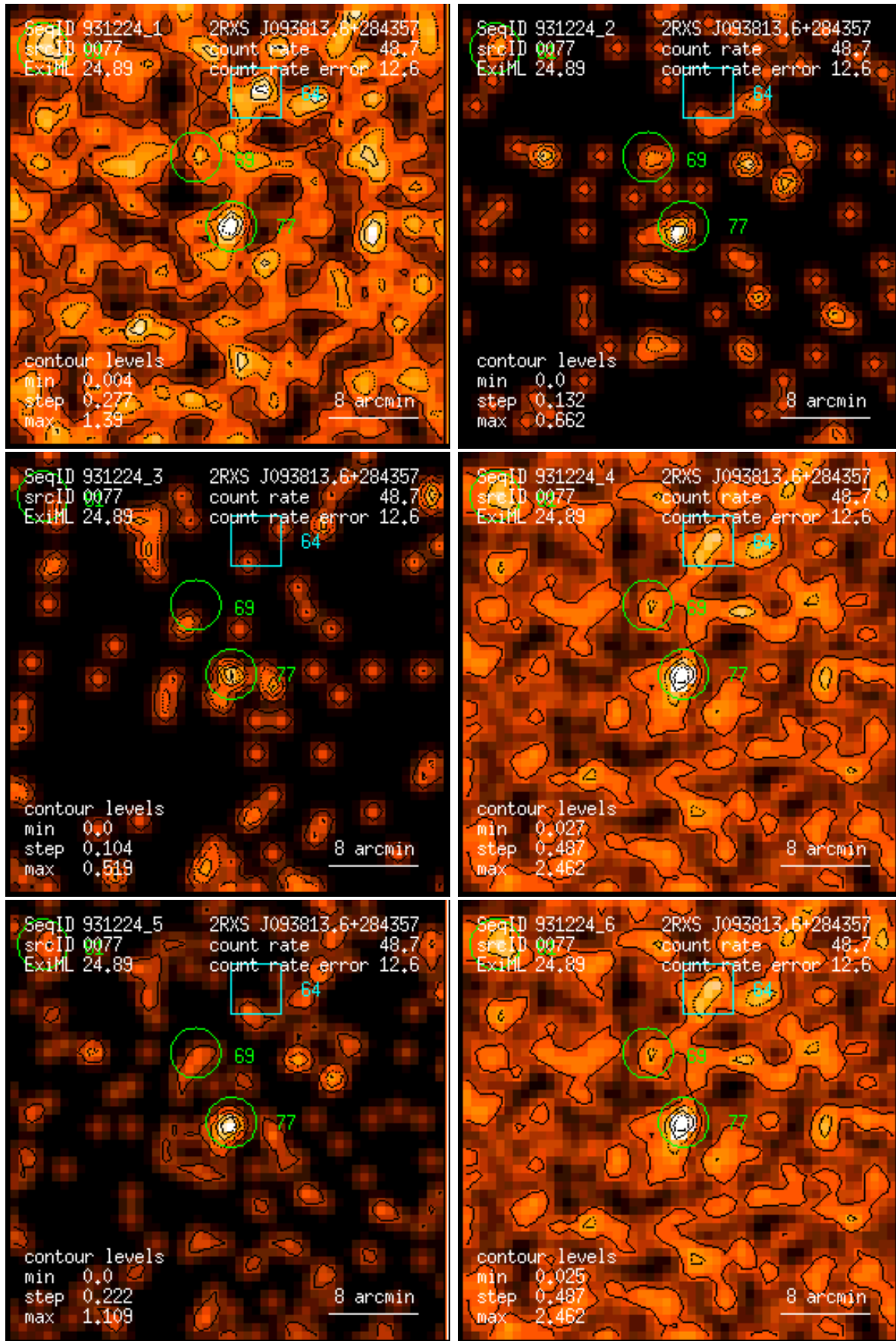
Figure 77: RASS 931224: detection 0077: band rate images, Gaussian filter: (1) PSPC channels 11 – 41, (2) 52 – 90, (3) 91 – 201, (4) 11 – 235, (5) 52 – 201, (6) 11 – 201. Broad band rates in counts/ks. Band rate contour levels in counts/ks/arcmin 2 .
