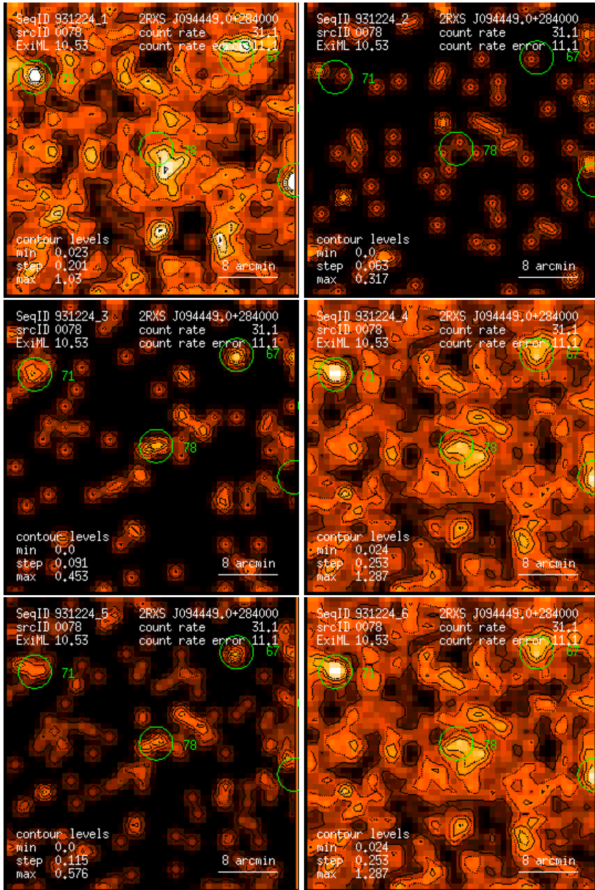
Figure 78: RASS 931224: detection 0078: band rate images, Gaussian filter: (1) PSPC channels 11 – 41, (2) 52 – 90, (3) 91 – 201, (4) 11 – 235, (5) 52 – 201, (6) 11 – 201. Broad band rates in counts/ks. Band rate contour levels in counts/ks/arcmin 2 .
