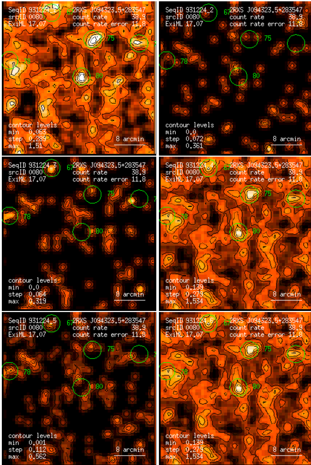
Figure 80: RASS 931224: detection 0080: band rate images, Gaussian filter: (1) PSPC channels 11 – 41, (2) 52 – 90, (3) 91 – 201, (4) 11 – 235, (5) 52 – 201, (6) 11 – 201. Broad band rates in counts/ks. Band rate contour levels in counts/ks/arcmin 2 .
