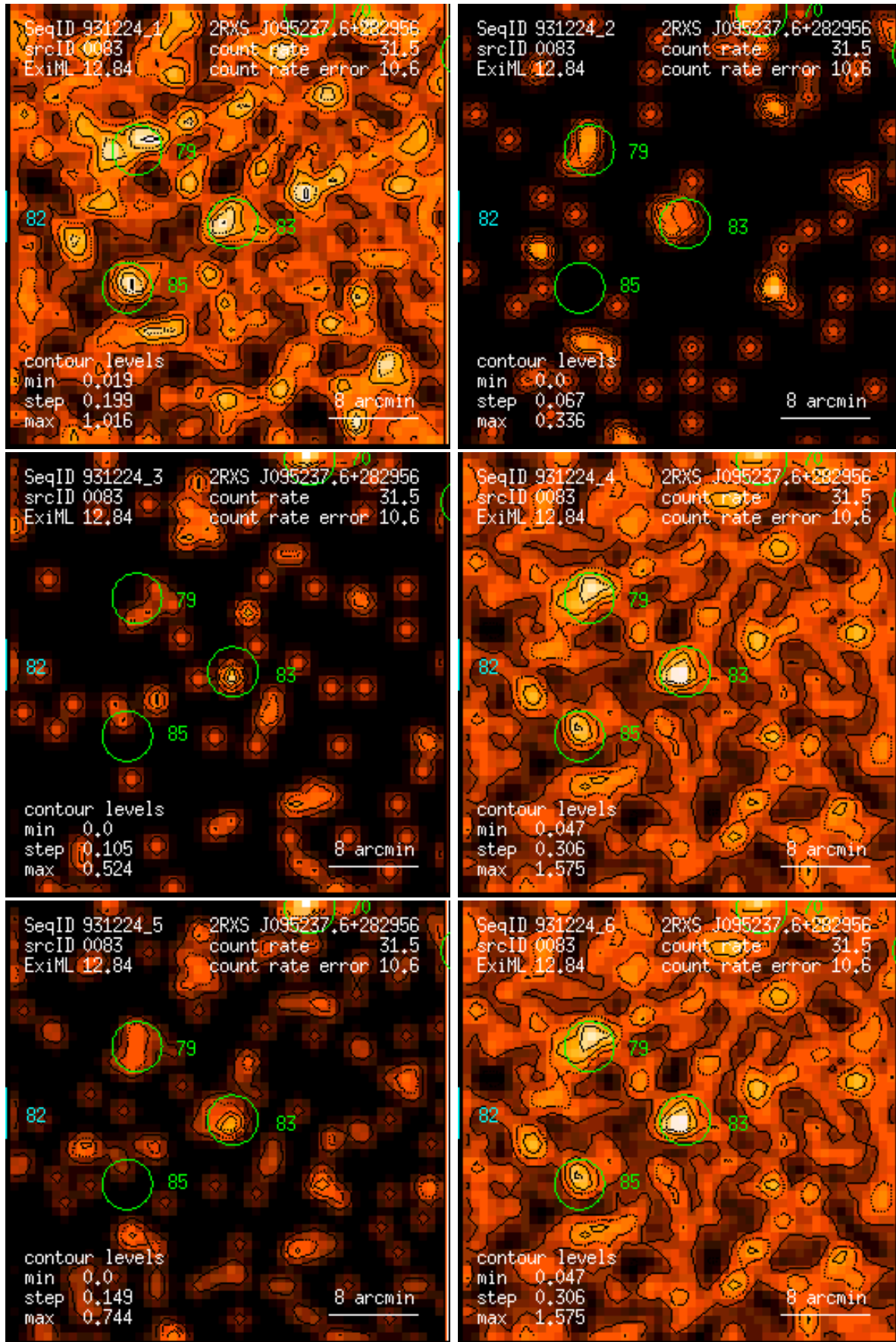
Figure 83: RASS 931224: detection 0083: band rate images, Gaussian filter: (1) PSPC channels 11 – 41, (2) 52 – 90, (3) 91 – 201, (4) 11 – 235, (5) 52 – 201, (6) 11 – 201. Broad band rates in counts/ks. Band rate contour levels in counts/ks/arcmin 2 .
