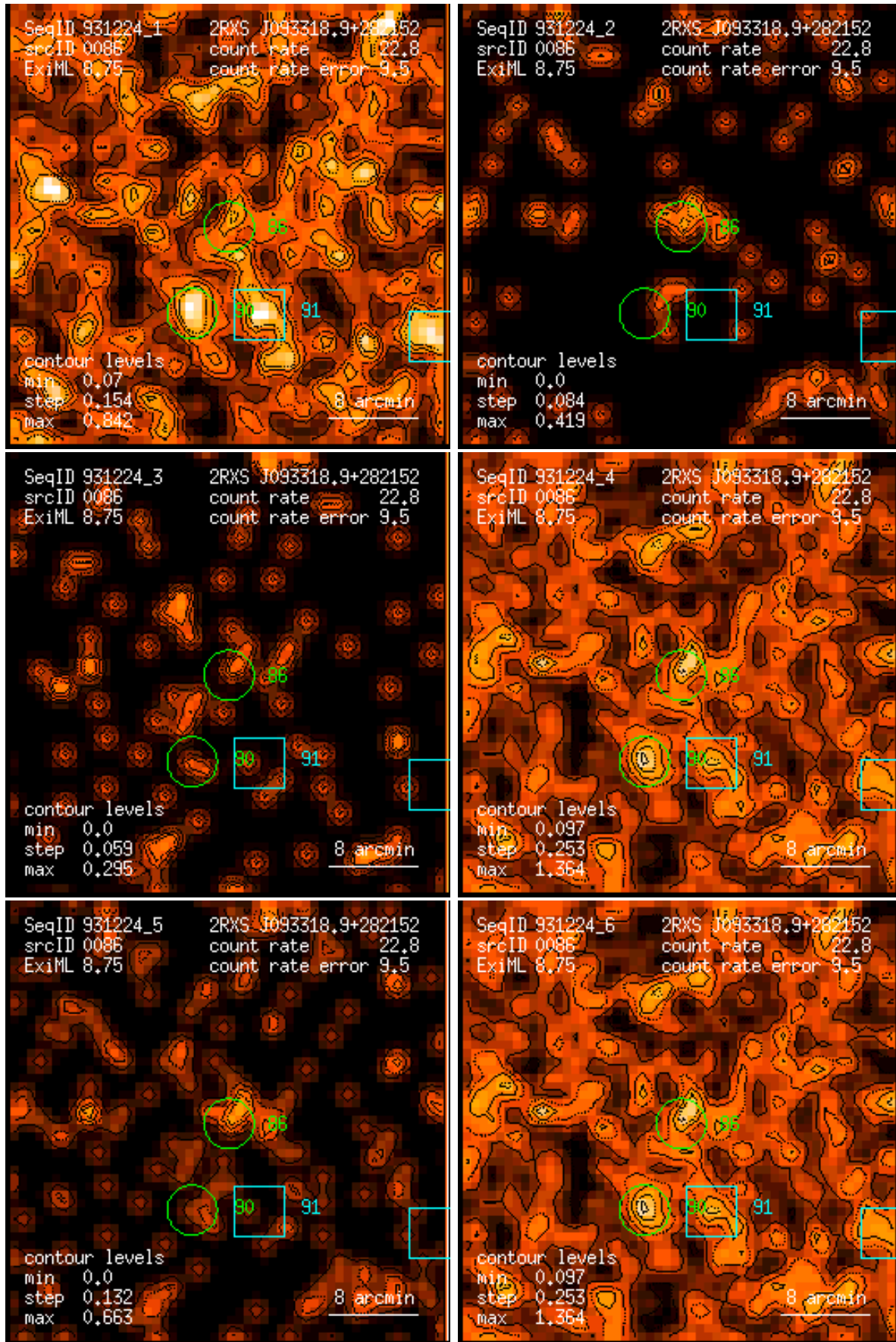
Figure 86: RASS 931224: detection 0086: band rate images, Gaussian filter: (1) PSPC channels 11 – 41, (2) 52 – 90, (3) 91 – 201, (4) 11 – 235, (5) 52 – 201, (6) 11 – 201. Broad band rates in counts/ks. Band rate contour levels in counts/ks/arcmin 2 .
