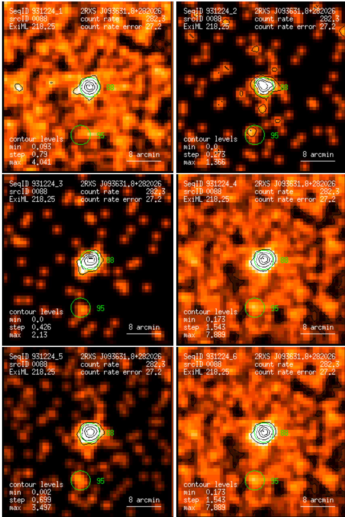
Figure 88: RASS 931224: detection 0088: band rate images, Gaussian filter: (1) PSPC channels 11 – 41, (2) 52 – 90, (3) 91 – 201, (4) 11 – 235, (5) 52 – 201, (6) 11 – 201. Broad band rates in counts/ks. Band rate contour levels in counts/ks/arcmin 2 .
