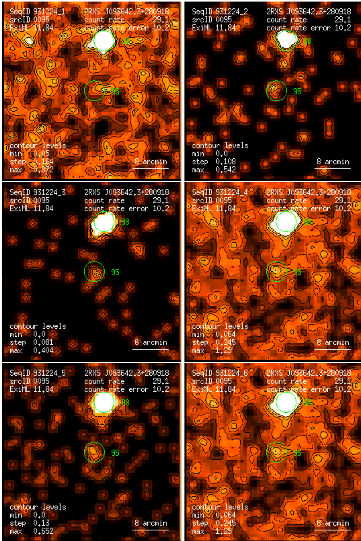
Figure 95: RASS 931224: detection 0095: band rate images, Gaussian filter: (1) PSPC channels 11 – 41, (2) 52 – 90, (3) 91 – 201, (4) 11 – 235, (5) 52 – 201, (6) 11 – 201. Broad band rates in counts/ks. Band rate contour levels in counts/ks/arcmin 2 .
