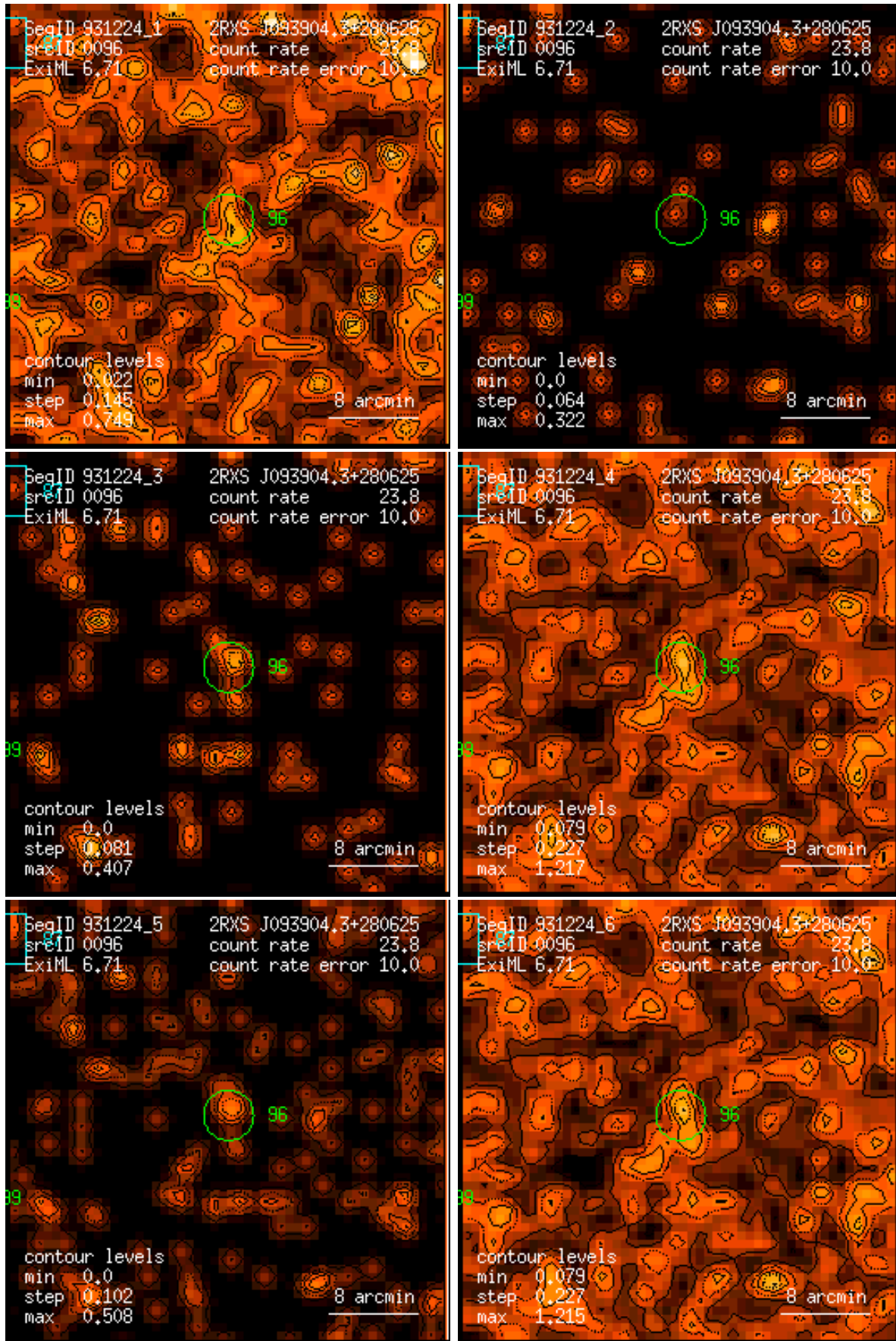
Figure 96: RASS 931224: detection 0096: band rate images, Gaussian filter: (1) PSPC channels 11 – 41, (2) 52 – 90, (3) 91 – 201, (4) 11 – 235, (5) 52 – 201, (6) 11 – 201. Broad band rates in counts/ks. Band rate contour levels in counts/ks/arcmin 2 .
